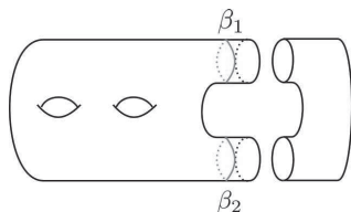
Figure 1: Essential simple closed curves \beta_1, \beta_2 parallel to the boundary components.
