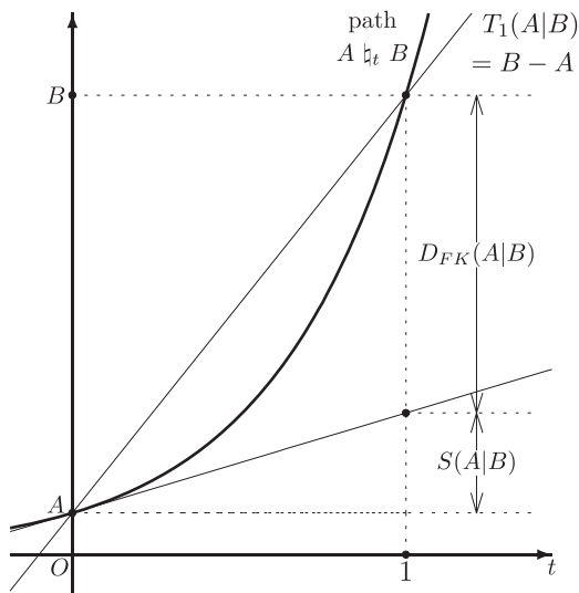
Figure 2. An interpretation of D_{FK}^{[n]}(A|B) .
