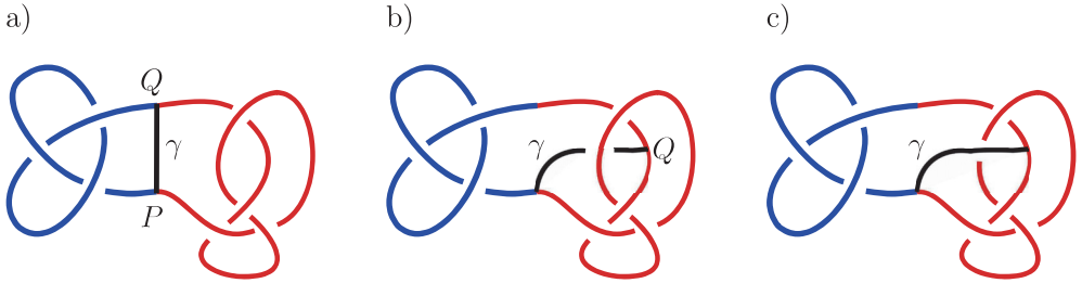
Figure 3: a) For this choice of P and Q the black arc \gamma minimizes c(D') because it does not add any crossings to D . The constituent knots of this theta curve are 3_1 \# 4_1 , 3_1 and 4_1 . b) For a different choice of P and Q the black arc has to intersect D somewhere. The shown arc does so the minimal number of times possible. The constituent knots of this theta curve are 3_1 \# 4_1 , 3_1 and 4_1 . c) Changing the signs of crossings between the black arc and the diagram D does not change the fact that \gamma minimizes c(D') for this choice of endpoints P and Q . It can change the constituent knots however. Here they are 3_1 \# 4_1 , 3_1 and the unknot.
