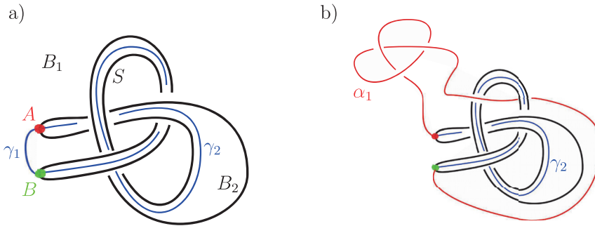
Figure 1: a) The path \gamma_1 is minimal in B_1 with c(\gamma_1) = 0 . The path \gamma_2 is minimal in B_2 with c(\gamma_2) = 3 . The path \gamma_2 is isotopic to a path in S = \partial B_2 = \partial B_1 , while \gamma_1 is not. b) The path \gamma_2 is minimal in B_2 with respect to \alpha_1 with c(\gamma_2 \cup \alpha_1) = 6 and is isotopic to a path in S .
