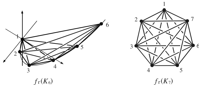
Figure 4: Standard rectilinear spatial graphs of K_n ( n = 6, 7 )
