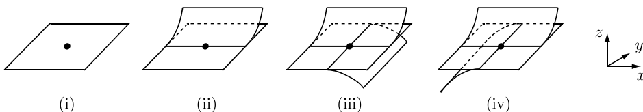
Figure 5: The local models of a flow-spine.
