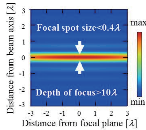
径偏光・狭リング形状ビームを集光した時の焦点近傍の光強度分布 (λは波長を表す) Intensity profiles of a radially polarized halo shape beam near the focal plane
