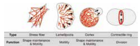
動物細胞で見られる様々な種類の細胞骨格の模式図 Schematic illustrations of various types of cytoskeleton in animal cells
