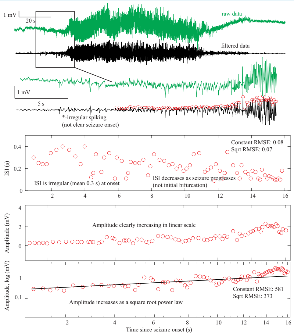
Appendix 1—figure 2. Supercritical Hopf Onset DC-coupled recordings (green, top) do not have a DC shift at onset. The ISI is arbitrary at onset, then after 10 s starts to decrease (middle). This irregular spiking prior to the seizure (*) is not part of a clear seizure onset, does not conform to any initial bifurcation, and thus was not chosen as the unequivocal seizure onset. The sustained spiking that begins at 8 s, however, follows the SupH dynamics very well. Amplitude shows steady increase in linear scale, which appears as a straight light in loglog plots, consistent with a square root power law (loglog plot). This seizure is most consistent with SupH due to the amplitude scaling. Onset Classification: This onset is somewhat challenging because there was some disagreement about when the seizure started. A more straightforward SupH onset is seen in Figure 2 and Appendix 1—figure 8 . In this case, two reviewers felt the irregular spiking was not a sustained start of the seizure and potentially was just preictal. One reviewer thought it could be the start and the seizure might be an arbitrary pattern (SubH or SN (-DC)). After discussion, reviewers agreed that the primary sustained pattern was increasing amplitude. Final analysis—DC shift: no. Amplitude increasing: yes, therefore SupH onset, but with note made of irregular spiking at seizure onset of uncertain significance. Offset Classification: This offset is difficult because there is decreasing amplitude like the onset, but then a persistent low voltage fast activity. DC shift: no. Amplitude decreasing: There was disagreement about whether the decrease comprised the final dynamotype of the seizure terminus, or if the low voltage fast activity that persisted at the end was a separate pattern. ISI increasing: no. Thus there was disagreement about
