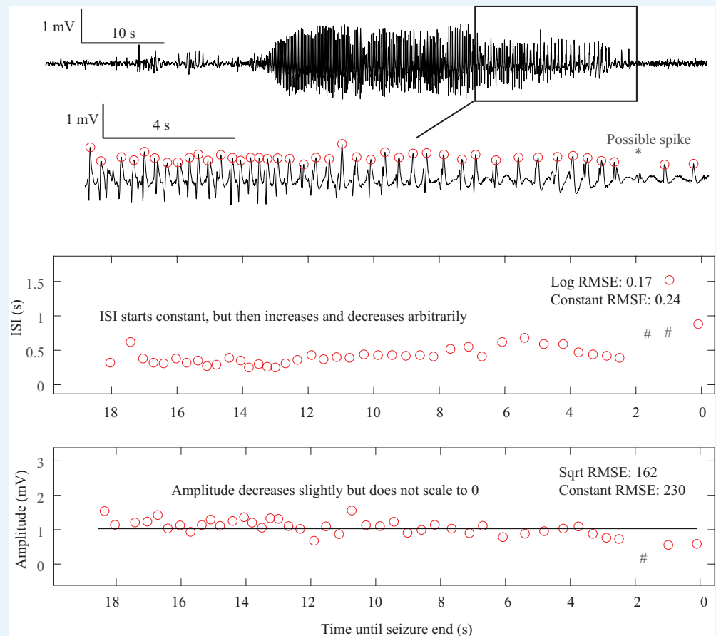
Appendix 1—figure 9. Fold Limit Cycle offset. The primary feature of the FLC is the lack of scaling laws. In this case, the ISI is constant until 8 s prior to the termination, then begins to increase until 6.5 s, then decreases until 2 s, then increases again. Even if including the one low-amplitude ‘failed’ spike at the *, the ISI is still arbitrary and does not follow log or square root scaling laws (#- location of ISI if the extra spike is included). The end of the seizure is abrupt. This arbitrary pattern is consistent with FLC offset. Other examples of FLC-terminal seizures are shown in Appendix 1—figures 3, 6, 10, 17 . Offset Classification: DC shift: no. Amplitude decreasing: no. ISI increasing: no (not consistent). Thus, this is a FLC offset. Onset Classification: No consensus, as it had ambiguous onset time. If it started early it could be a SN-(DC) or SubH, or if it started later it could be a SupH.
