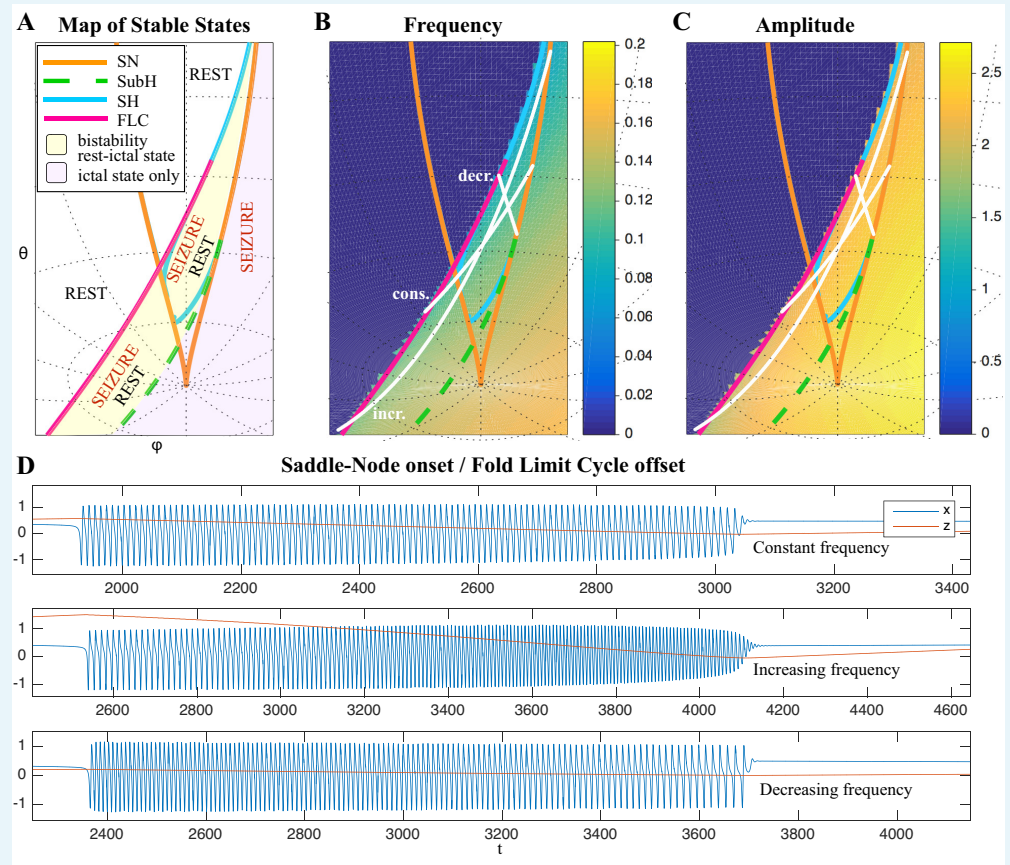
Appendix 1—figure 18. Varied frequency behavior of FLC offsets. Depending on how close the trajectory comes to the SH offset, an FLC offset can have a wide range of frequency behaviors. We show examples for three frequency trends for the FLC bifurcation. (A) Portion of the map in which the SubH/FLC type can be found. (B–C) Frequency and amplitude trajectories of three different seizures showing constant, increasing, and decreasing frequency. (D) Simulations for the paths shown in B–C. Note the last few spikes drop in amplitude precipitously, characteristic of the FLC releasing from the limit cycle (which has a finite amplitude when it disappears) and settling on the fixed point. This is different from the square-root decreasing amplitude of the SupH bifurcation, which is instead caused by a slow decrease in the amplitude of the limit cycle itself, in this latter case the limit cycle disappears when zero amplitude is reached.
