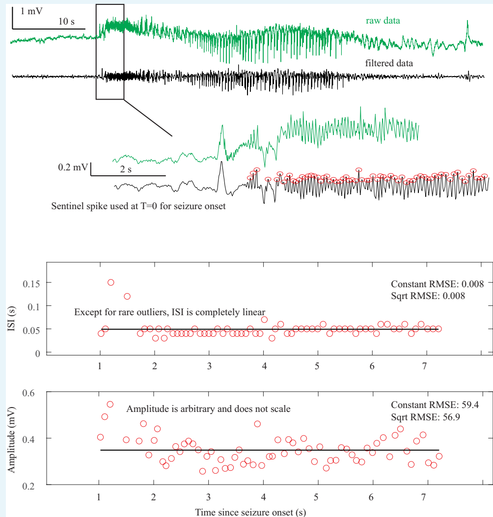
Appendix 1—figure 1. Saddle Node Onset DC-coupled recordings (green, top) show DC shift that occurs immediately upon seizure onset. To determine spike amplitudes and ISI, data must be high-pass filtered (black). Those filtered data are then used to identify the spikes (red circles) for analysis. The interspike intervals (ISI, middle) and amplitude (bottom) of each spike are then plotted versus time since seizure onset for visual analysis and curve fitting. The seizure begins with fast 20 Hz firing at arbitrary amplitude for over 5 s. This is followed by changing amplitude, irregular firing, and then clonic bursting, but those are clearly after the initial onset. The combination of arbitrary amplitude, ISI, and DC shift is consistent with Saddle Node. Onset Classification: DC shift: yes, therefore SN onset. All three reviewers agreed. Offset Classification: 57640 This is an example of a challenging offset. Analysis is uncertain because seizure offset time is unclear (is it when the fast spikes stop, when the slower oscillations stop, when the low voltage fast activity stops, or when the large final spike occurs?). Thus, the method is uncertain. DC shift: no. Amplitude decreasing: uncertain. ISI increasing: uncertain. This offset is ambiguous and reviewers were unable to reach consensus. One reviewer felt the high amplitude spiking fit with increasing ISI (SH or SNIC). Another felt it should be FLC because of the arbitrary patterns. Another was uncertain how to score given the ambiguity of seizure offset. It was listed as ‘no consensus’.
