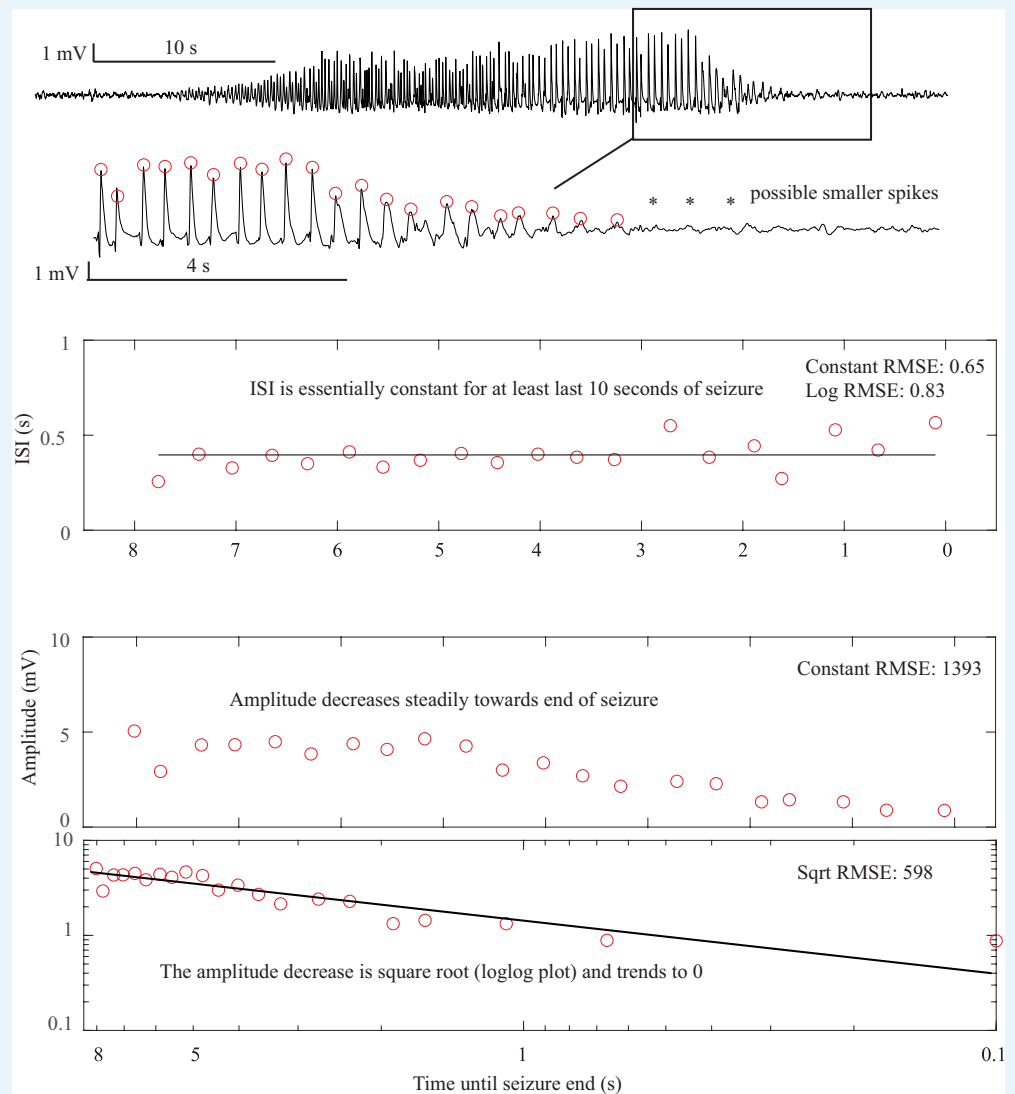
Appendix 1—figure 8. Supercritical Hopf onset and offset. This is the seizure from Figure 2D . Here, the terminal ISI is nearly constant and does not have any ‘slowing down.’ The amplitude, on the other hand, clearly diminishes and trends to zero as a square root power law by the end of the seizure. There are even some potential smaller spikes seen after the seizure (*), as if the spikes have vanished into the background noise. In this case, the seizure stops because the amplitude, rather than the frequency, has gone to zero. The constant ISI and diminishing amplitude are indicative of the SupH offset. The same pattern occurs at onset. Offset Classification: DC shift: no. Amplitude decreasing: yes. This is a SupH offset. The ISI is also constant, which is consistent but not necessary for the classification due to prioritization. Onset Classification: DC shift: no. Amplitude increasing: yes. This is a SupH onset.
