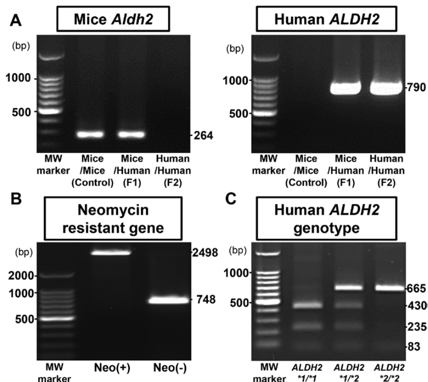
Figure 2. Genotyping of human ALDH2*1/*1 , ALDH2*1/*2 and ALDH2*2/*2 knock-in mice. (A) PCR images for mice Aldh2 (left panel), and human ALDH2 (right panel). Left lane in left and right panel: molecular weight (MW) marker, 100 base pair (bp) DNA ladder. PCR products of mice Aldh2 and human ALDH2 were 264 bp and 790 bp, respectively. (B) Elimination of neomycin resistant gene. Left lane: MW marker (100 bp DNA ladder). PCR products of human ALDH2 with or without neomycin-resistant gene were 2498 bp and 748 bp, respectively. Neo (+): before elimination of neomycin resistant gene, Neo (-): after elimination of neomycin resistant gene. (C) The PCR images (PCR-RFLP methods) for ALDH2*1/*1 , ALDH2*1/*2 and ALDH2*2/*2 mice. Left lane: MW marker (100 bp DNA ladder). Digestion of PCR products with AcuI harbored three bands (430, 235 and 83 bp) in ALDH2*1/*1 mice, four bands (665, 430, 235 and 83 bp) in ALDH2*1/*2 mice and two bands (665 and 83 bp) in ALDH2*2/*2 mice.
