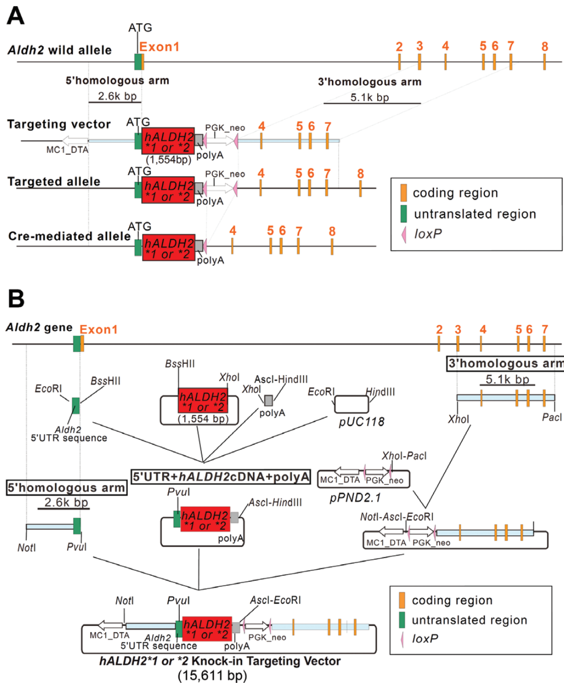
Figure 1. Scheme of human ALDH2*1 or ALDH2*2 targeting vector to generate genetically engineered knock-in mice that express the human ALDH2*1 or ALDH2*2 gene. (A) Human ALDH2 (ALDH2*1 or ALDH2) cDNA knock-in strategy. bp: base pair. (B) Construction for human ALDH2*1 or ALDH2*2 knock-in targeting vector. 5' homologous arm (2.6k bp), 5' UTR of exon 1 of Aldh2 gene + human ALDH2 (ALDH2*1 or ALDH2) cDNA (1554 bp) + polyA containing vector, and 3' homologous arm (5.1k bp) are included in human ALDH2*1 or ALDH2*2 knock-in targeting vector.
