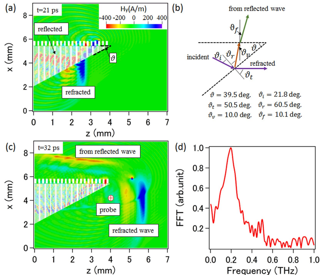
Figure 4. (a) Simulation results for the contour map of the y-directed magnetic field at t = 21 ps. (b) Schematic diagram of the radiation scheme. (c) Simulation results for the contour map of the y-directed magnetic field at t = 32 ps. (d) Radiation spectrum observed at the probe point.
