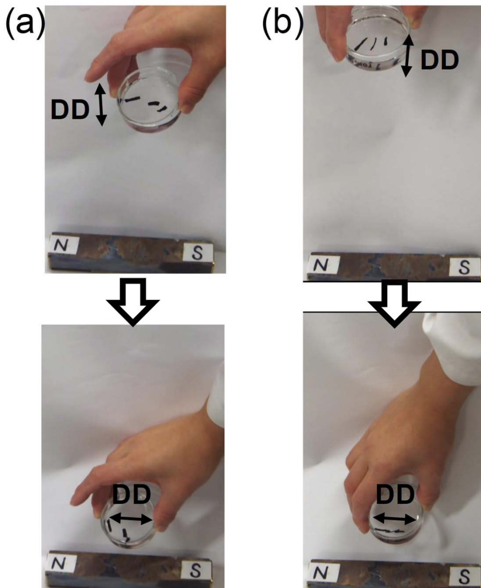
2 Figure 7 Photographic data showing magnetic orientation behavior of Car/PVA/Fe 3 rectangular strips cut from a drawn sheet (draw ratio, three times): DD was (a) 4 perpendicular and (b) parallel to the longer axis of the strips. The strips were floated on 5 ethanol in a glass dish.
