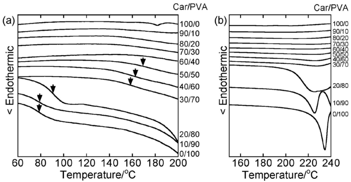
3 Figure 1 DSC thermograms of Car/PVA composites in the second heating scan. Mid- 4 point T_g positions are indicated by arrows for the respective compositions in (a). Part 5 (b) represents enlarged thermograms around the melting point of PVA.
