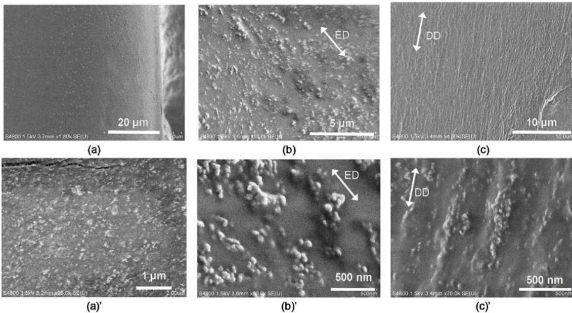
8 Figure 2 FE-SEM images for the surfaces of (a) as-cast, (b) as-spun, and (c) drawn 9 (four times) sheets of Car/PVA/Fe. The image with the prime symbol shows each 10 enlarged view.
