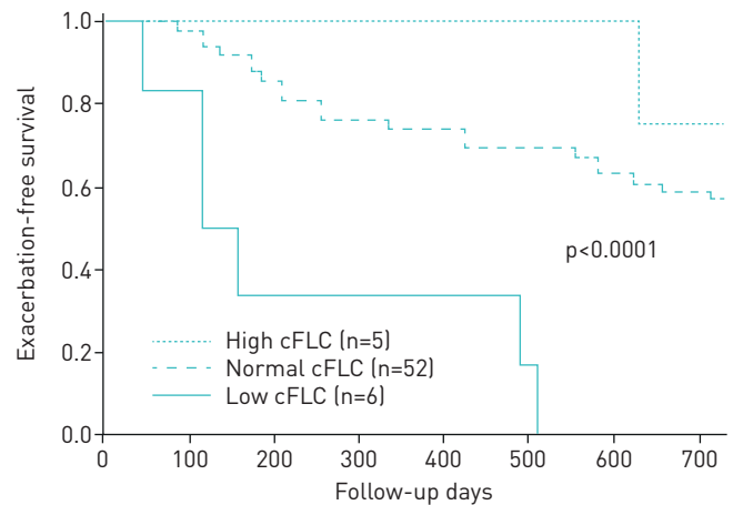
FIGURE 2 Kaplan–Meier curve for the time to the first moderate/severe exacerbation based on combined free light chain (cFLC) subgroups. The patients with low cFLC (solid line, n=6 ) showed significantly shorter time to the first exacerbation of COPD than patients with normal (dashed line, n=52 ) or high cFLCs (dotted line, n=5 ) ( p<0.0001 by log-rank test).
