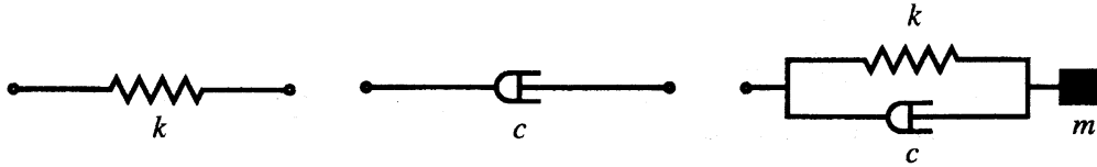
Figure 1: A spring, a dashpot, and the Voigt model
