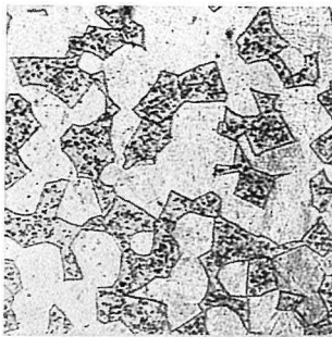
Photo 23. 6.1% Al Quenched from 700°C in ice- water, after annealing for 2 hrs. at 700°C.
