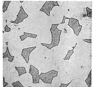
Photo 27. 6.1% Al Slowly cooled to 610°C after annealing for 2 hrs. at 700°C and quenched from 610°C in ice-water.
