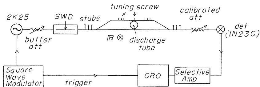
Fig. 1. Block diagram of the apparatus.
