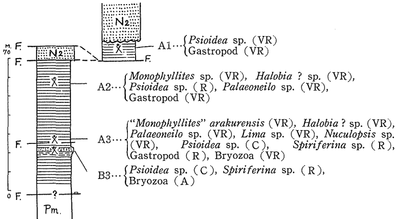
Fig. 17. Columnar sections of the Arakura formation.
