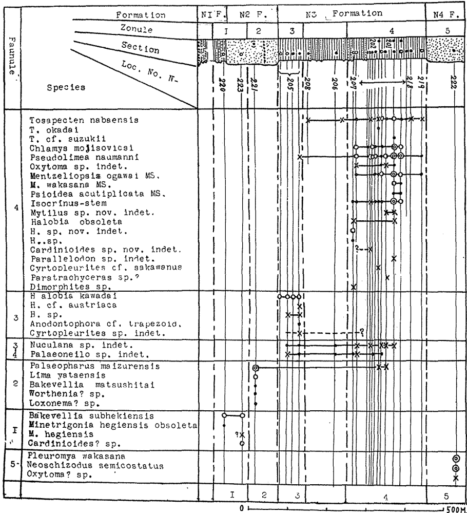
Fig. 18. Range-chart of species of the Nabae group in the Nabae district.
