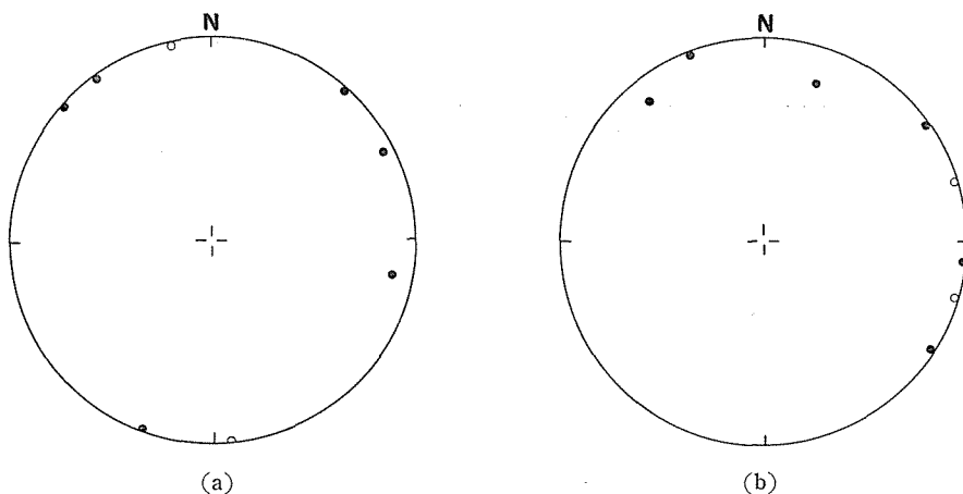
Fig. 1. Direction of magnetization of crystalline schists with (a) "magnetite" and (b) "hematite". The equatorial plane of this Schmidt's projection is the plane of schistosity. Hollow circles represent positive magnetic poles appearing on upper hemisphere. Full circles represent positive magnetic poles appearing on lower hemisphere.
