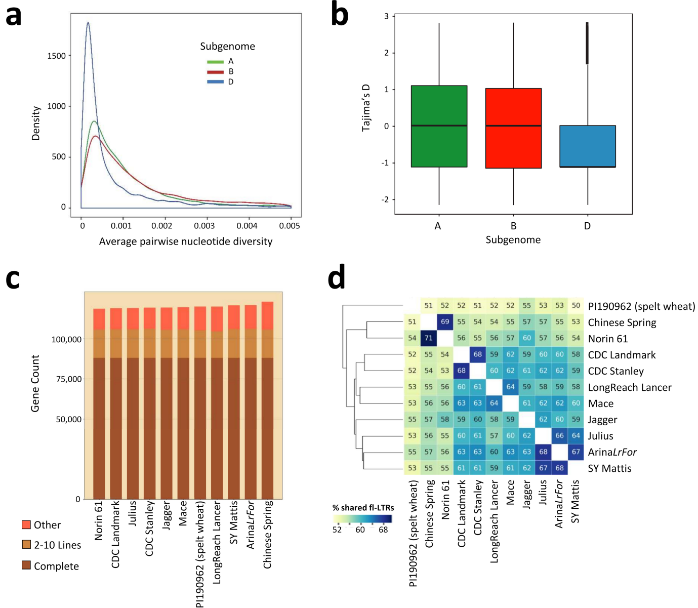
Extended Data Fig. 3 | Diversity of genes and TEs. a , Average pairwise genetic diversity of the homeologues (coding sequences only) of the A, B and D subgenomes. The mode of the A, B and D subgenome is 0.00057, 0.00082, and 0.0002, respectively. b , Tajima's D estimates of coding sequences for each wheat subgenome. The lower and upper range of the boxplot hinges correspond to the first and third quartiles (the 25th and 75th percentiles). Boxplots show centre line, median; box limits, upper and lower quartiles;
