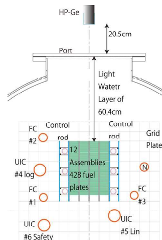
Fig. 1 Experimental setup
