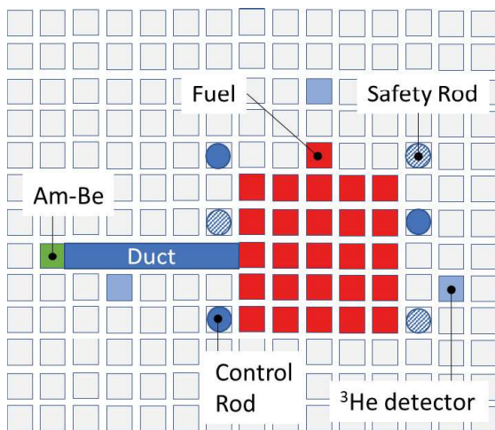
Fig. 1. Configuration of fuels and devices in A-core.
