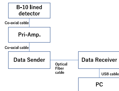
Fig.2 Data transfer system
