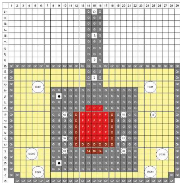
Fig. 1 Core configuration (B7/4”G2/8”p8EUNU+3/8”p38EU)
