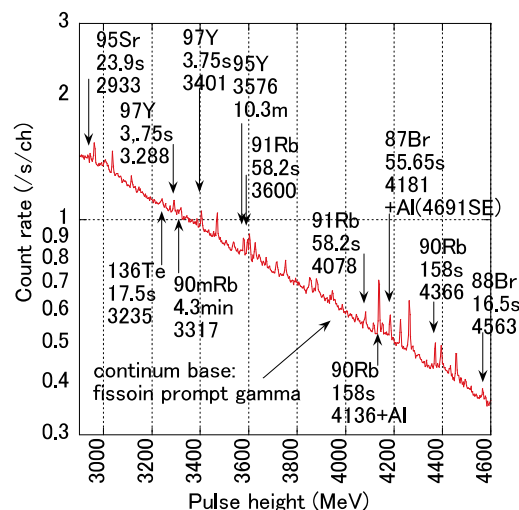
Fig. 2 \gamma rays from short lived FP measured for critical core (C35 U-assembly)
