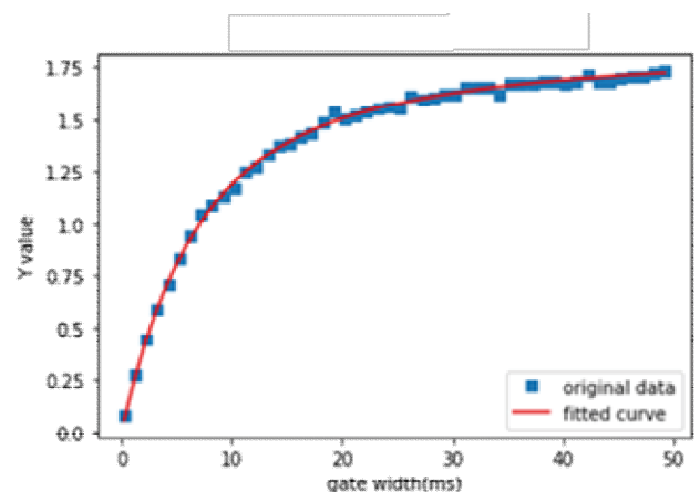
Fig 3: Example of present Feynman- Y curve.
