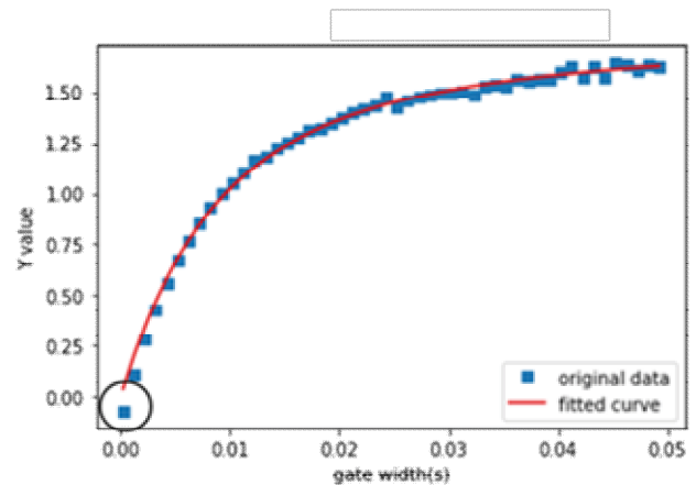
Fig. 1: Example of conventional Feynman- Y curve.
