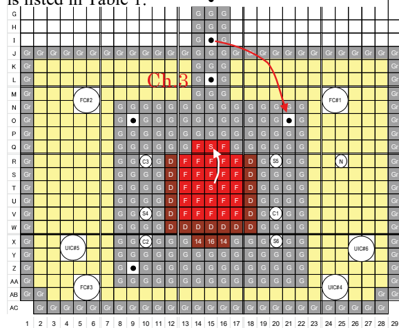
Fig. 1. Core configuration.
