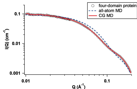
Fig. 1. SAXS profile of four-domain protein (circle). The dotted and continuous lines correspond to the calculated SAXS profile from the snapshot from all-atom MD and CG MD simulation, respectively.
