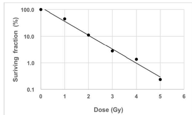
Fig. 1. Surviving fraction of the cells irradiated with the reactor neutrons.
