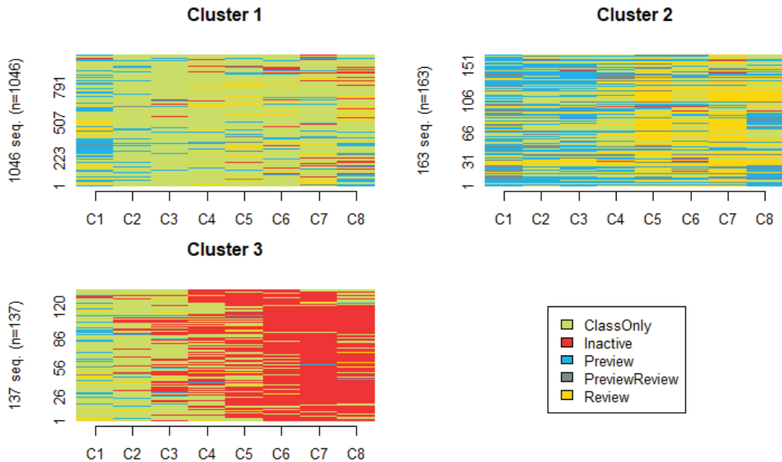
Figure 3. Distribution of Study Activities in each Cluster.
