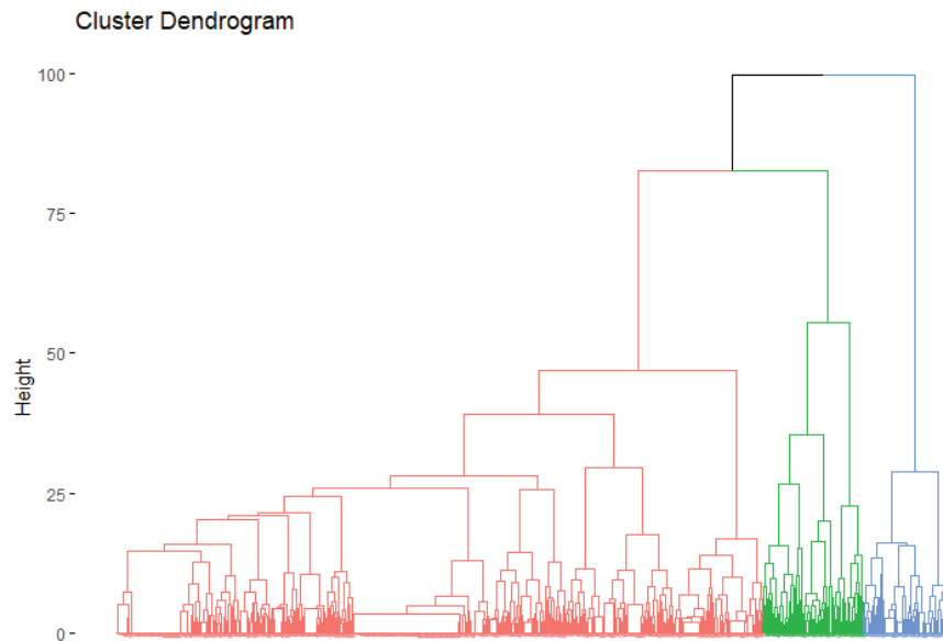
Figure 2. Dendrogram of the Hierarchical Cluster Analysis.
