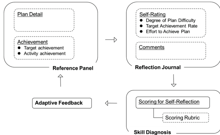
Figure 3. Self-Reflection Model
