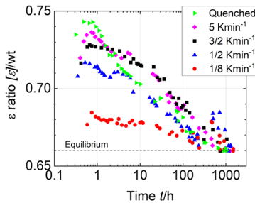
Fig. 2-2. Variations of weight fraction for \varepsilon phase.
