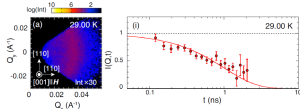
Fig. 3. Neutron scattering data of Skyrmion phase of MnSi just above the critical temperature. (Left) The diffuse scattering pattern on the Q_x - Q_y plane. (Right) I(Q, t) curve fitted by a single exponential function with time constant \tau = 1.02(5) ns [4].
