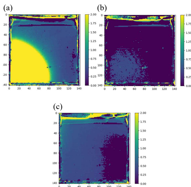
Fig. 1. A result for two-dimensional distributions: (a) thermal neutron component, (b) fast neutron component and (c) gamma ray component.
