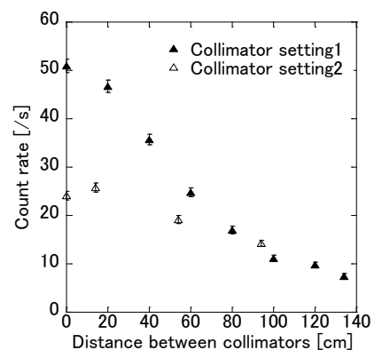
Fig. 3. Dependence of distance between collimators and 10 B count rate.
