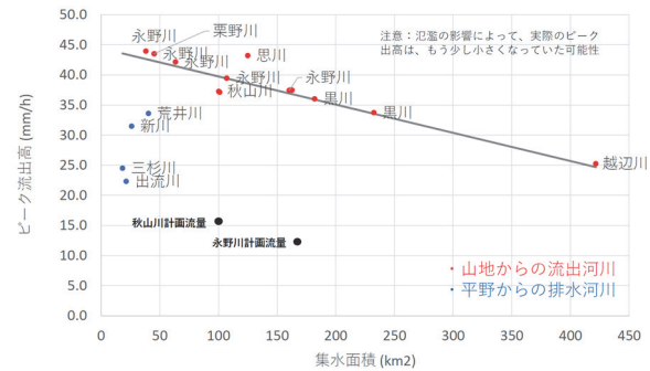
Fig. 7 Simulated peak runoff at levee breaching points in medium-to-small rivers in Tochigi prefecture (and Saitama prefecture for the Opepe river). The red points are rivers originated from mountains, while the blue points are rivers originated from plains
