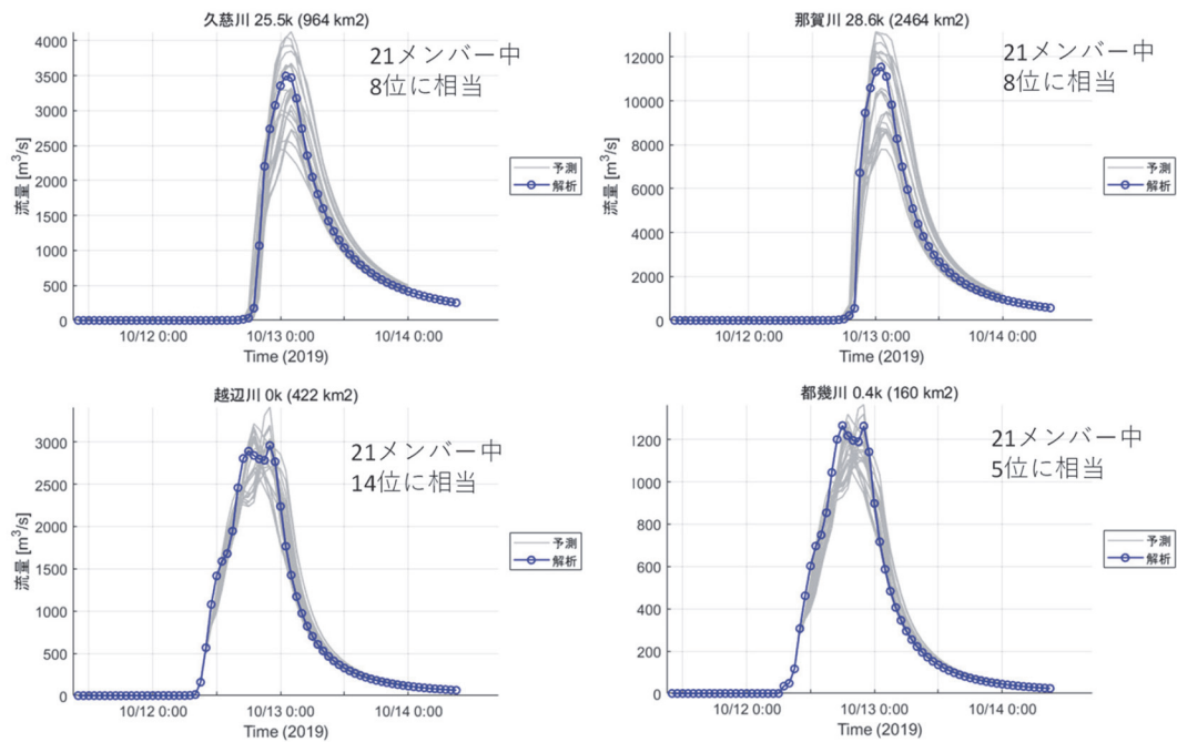
Fig. 13 Estimated discharge by the RRI model at Kuji, Naka, Ope and Toki (the upstream of Arakawa) rivers: 21 members based on the MEPS input (gray) and analysis rainfall (blue)
