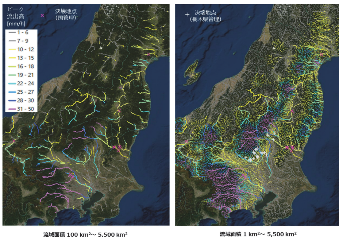
Fig. 10 The spatial distributions of the forecasted peak runoff (ensemble mean) based on MEPS and RRI with initial time at 9 am on October 11. Left: only along the main rivers, Right: for all rivers.
