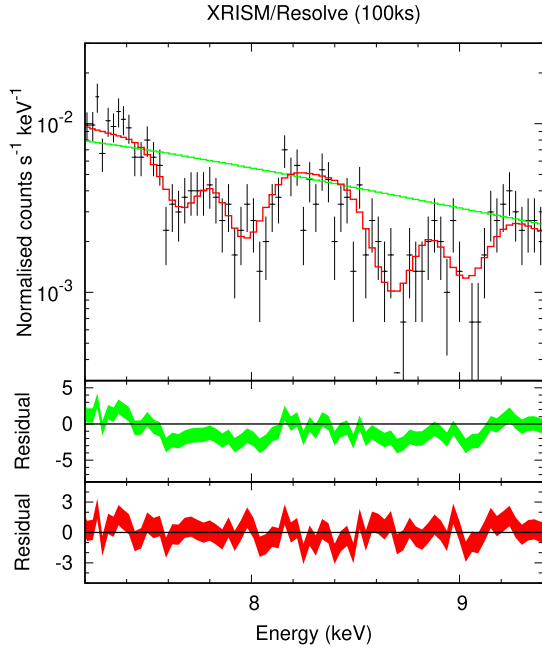
Figure 13. Same as Fig. 12, but for XRISM/Resolve.
