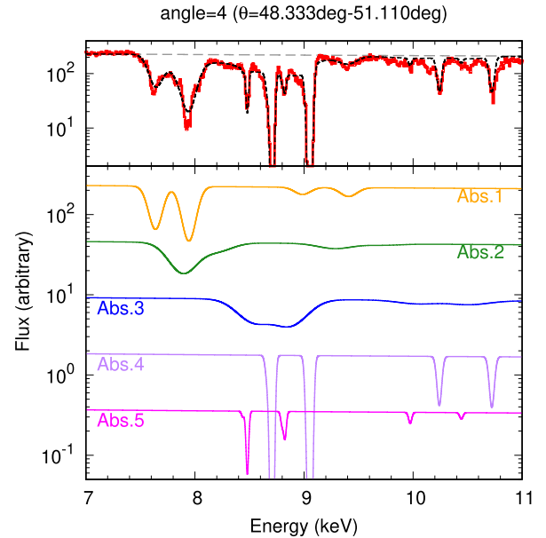
Figure 6. Upper panel: the primary spectrum (red, same as Fig. 4) is fitted by the power-law continuum with \Gamma = 2.2 . (grey dashed) and five photoionized absorbers (black dotted). Lower panel: absorption features produced by each photoionized absorber introduced. Each absorber has the iron Ly \alpha , Ly \beta and He \alpha , He \beta lines, which is modelled by the kabs model (Tomaru et al., in preparation). The free parameters are the number of H-like and He-like Fe ions ( N_{\text{atom}} ), velocity dispersion ( \sigma_v ), and wind velocity.
