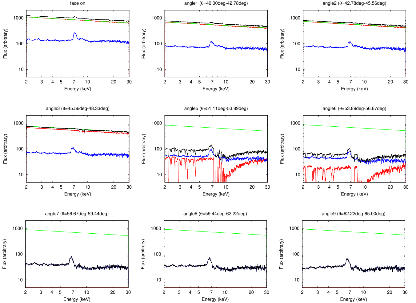
Figure 7. Synthesized X-ray spectra in all the viewing angle cases, except for angle4 (see Fig. 4).
