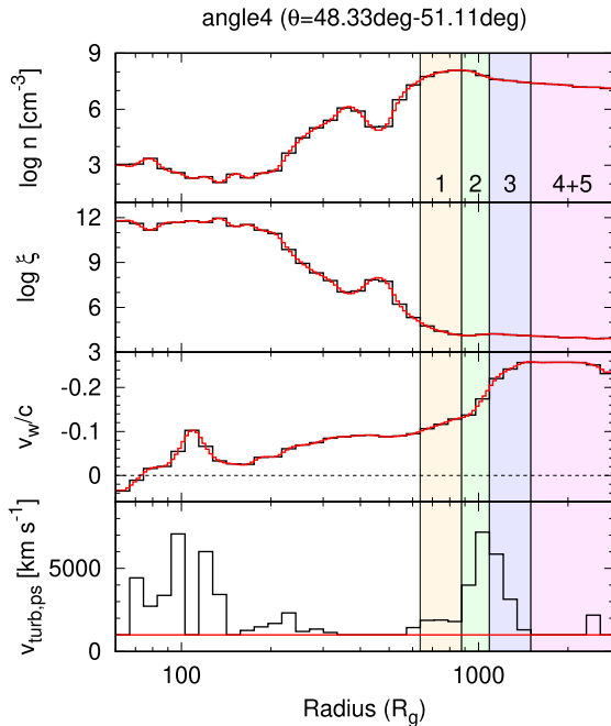
Figure B1. Radius dependence of the wind parameters (density, ionization parameter, velocity, pseudo-turbulent velocity) along angle4. The black lines are the same as those in the Fig. 5 in the main text. The red lines are the interpolated one, whose grids are four times as fine as the black ones. The pseudo-turbulent velocity in the red line is fixed as 1000 \text{ km s}^{-1} .
