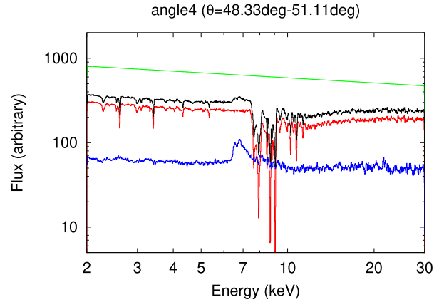
Figure 4. Synthesized X-ray spectra in the angle4 case. The vertical axis shows the arbitrary \text{keV}^2 flux. The red and blue lines show the primary and scattered spectra, respectively, and the black line is the total spectrum. The input power-law spectrum is shown in green.
