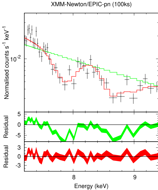
Figure 14. Same as Fig. 12, but for XMM-Newton/EPIC-pn .
