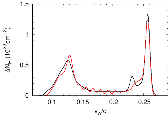
Figure B3. Column distributions against the wind velocity. The data in r > 600 R_g is used. The red line shows the fine grid case with v_{\text{turb}} = 1000 \text{ km s}^{-1} , whereas the black does the coarse grid case with v_{\text{turb}} = v_{\text{turb, ps}} .
