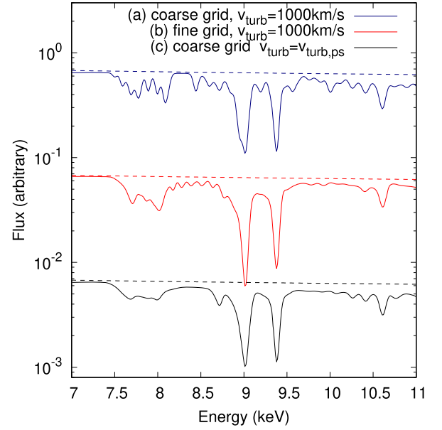
Figure B2. Spectral modelling for the wind along the line of sight. The dashed lines show the input power law.
