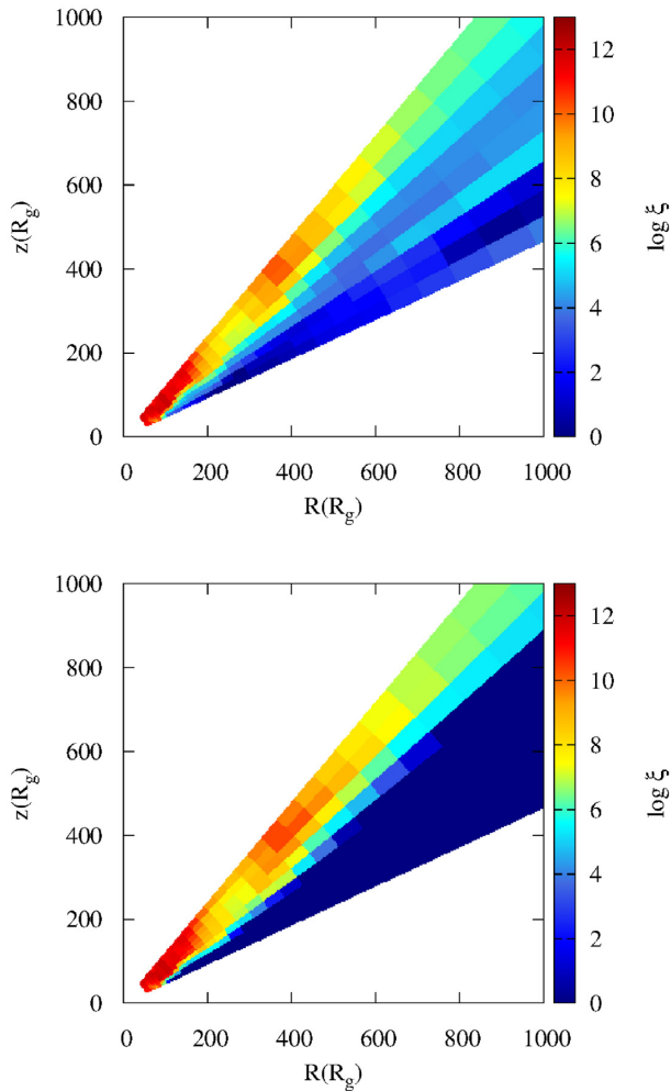
Figure 2. The upper panel shows the ionization parameter map used in the MONACO radiation transfer, recalculated from the original simulation using XSTAR. The lower panel shows the ionization parameter map from the original simulation of Nomura et al. (2020). Both share the same colour mapping. The underside of the wind (and its base) are slightly less ionized assuming full opacity than predicted from the step function, but the upper part of the wind where the UFO structures are seen are very similar in ionization state. We note that the region with \log \xi < 0 has the same colour as that with \log \xi = 0 , both of which have only the neutral Fe atoms.
