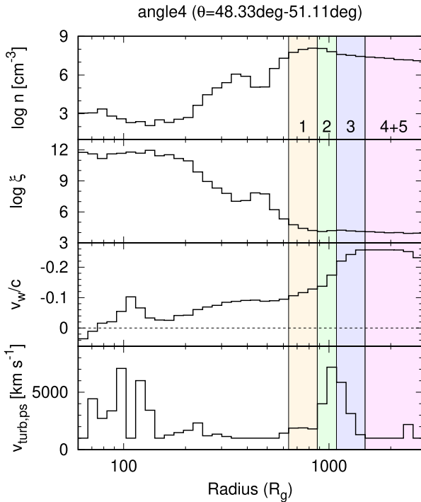
Figure 5. Radius dependence of the wind parameters (density, ionization parameter, velocity, pseudo-turbulent velocity) along angle4. The shaded regions potentially produce the UFO absorption lines. Each colour corresponds to each absorber component listed in Fig. 6 and Table 1.
