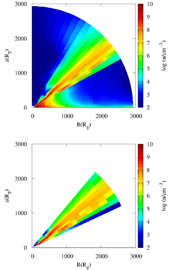
Figure 1. Density structure of the UV line-driven disc wind. The upper panel shows the original grid obtained from the radiation hydrodynamics simulation (Nomura et al. 2020), whereas the lower panel shows the resampled one.
