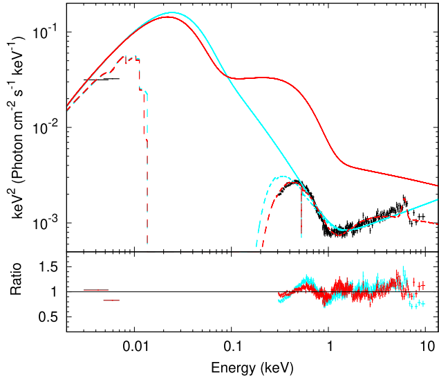
Figure 9. The broad-band SED of PG 1211+143 (ObsID=0112610101). The cyan lines show the naive fitting with the agns1im model, with \Gamma_{\text{hot}} = 1.6 . The solid line shows the intrinsic SED, whereas the dashed one is with the Galactic absorption. In order to set \Gamma_{\text{hot}} in a reasonable range for a high Eddington object, we introduce partial covering of neutral material, which is shown in red. We also take electron scattering due to the ionized wind into consideration. The lower panel shows ratios of the data to the model.
