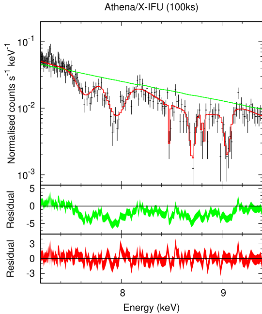
Figure 12. Simulated spectrum for 100-ks Athena /X-IFU observation. The green line shows the power-law continuum, and the red line shows the best fit of the photoionized absorber model. The middle and lower panels show residuals for the power-law model and the best-fitting photoionized absorber model, respectively.
