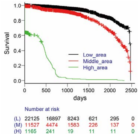
Fig. 3. Survival curves of Japanese Black cattle after the disaster by survey area.
