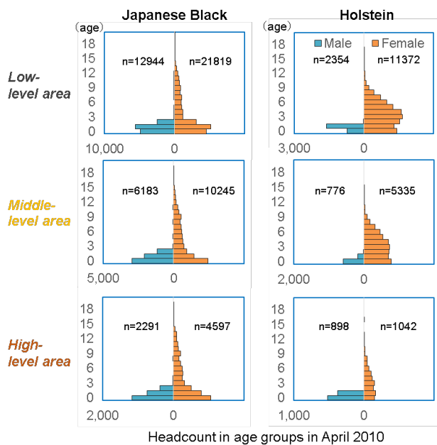
Fig. 2. Population pyramid of domestic cattle in a survey area in Fukushima Prefecture.
