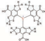
Figure 2. During the dynamic nuclear polarization process, polarization is transferred from the electrons of the doping material to the 13 C nuclei by means of microwave irradiation.
