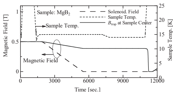
Fig. 3 Trapped magnetic field of MgB 2 sample.
