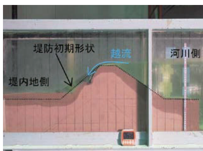
越流による河川堤防の堤体変形実験 Experiment on deformation of river dyke body due to overtopping flow
