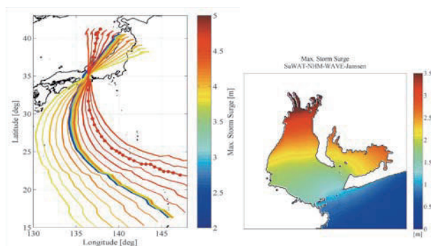
伊勢湾に來襲する台風の経路と高潮水位の関係 Simulated typhoon courses and storm surges modeled from the Isewan typhoon
