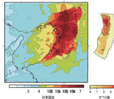
大阪平野下、上町断層帯の強震動予測 Ground motion prediction of an anticipated earthquake on Uemachi Fault system under Osaka Plain
