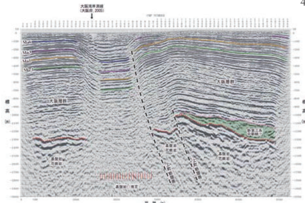
上町断層帯南部における反射法地震探査（堺一高石測線）結果と構造解釈 Geologic interpretation of the depth section by a seismic reflection survey across the Uemachi fault system
