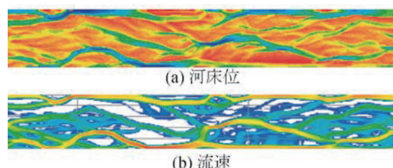
網状流路の数値解析 Numerical simulation of a braided stream
