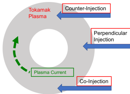
Fig. 1-8 Three injection geometries of NBI
