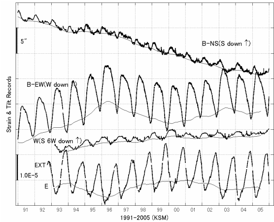
Fig.6 Secular variations of ground-strains and ground-tilts observed at the Kushima and Osumi Observatory. 365 days running mean of strains and tilts are also plotted in parallel.
