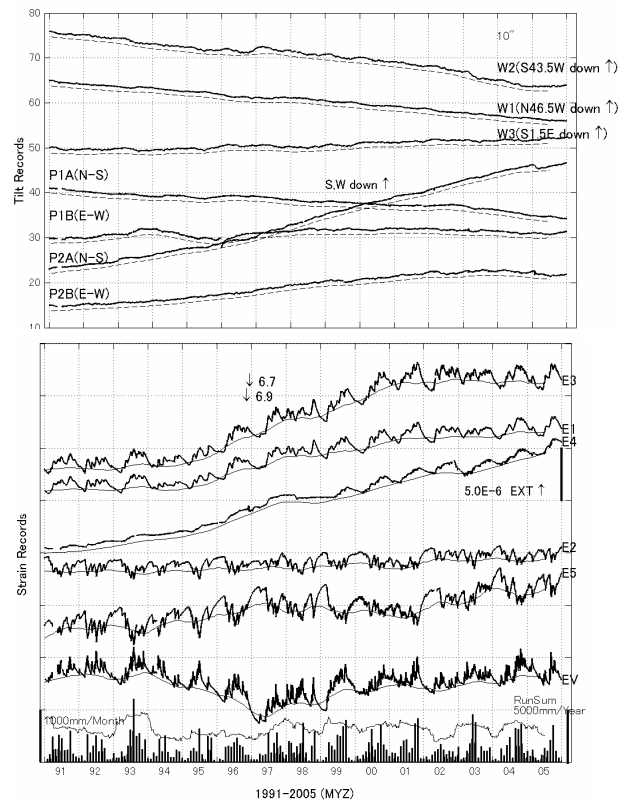
Fig.2 Secular variations of ground-strains observed with extensometers (E1~E5, EV), and ground-tilts observed with horizontal pendulum tiltmeter (P1,P2), Water-tube tiltmeters(W1~W3)at the Miyazaki Observatory. 365 days running mean of strains and tilts are also plotted in parallel.
