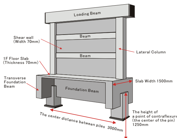
Fig.11 Specimen configuration
