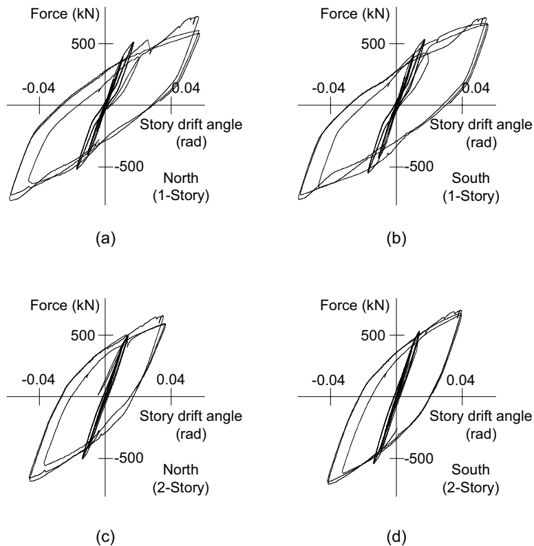
Fig. 10 Story shear versus story drift angle relationships up to 1/20 overall drift: (a) First story in “North” plane; (b) First story in “South” plane; (c) Second story in “North” plane; (d) Second story in “South” plane
