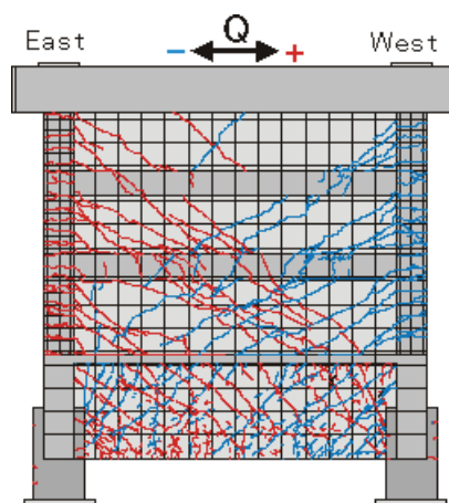
(a) Crack distribution
