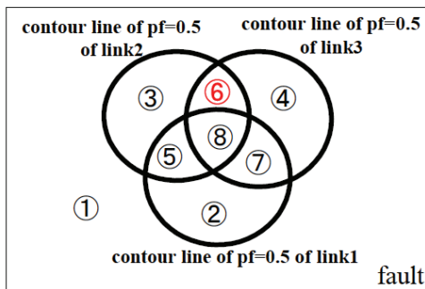
Fig. 21 Counter lines ( P_f=0.5 ) for 3 links
