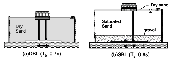
Fig. 15 Test models
