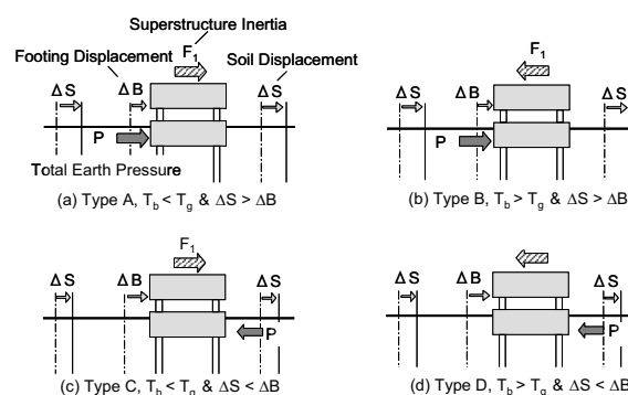
Fig. 17 Phase difference between total earth pressure and superstructure inertia (Tamura et al. 2002)
