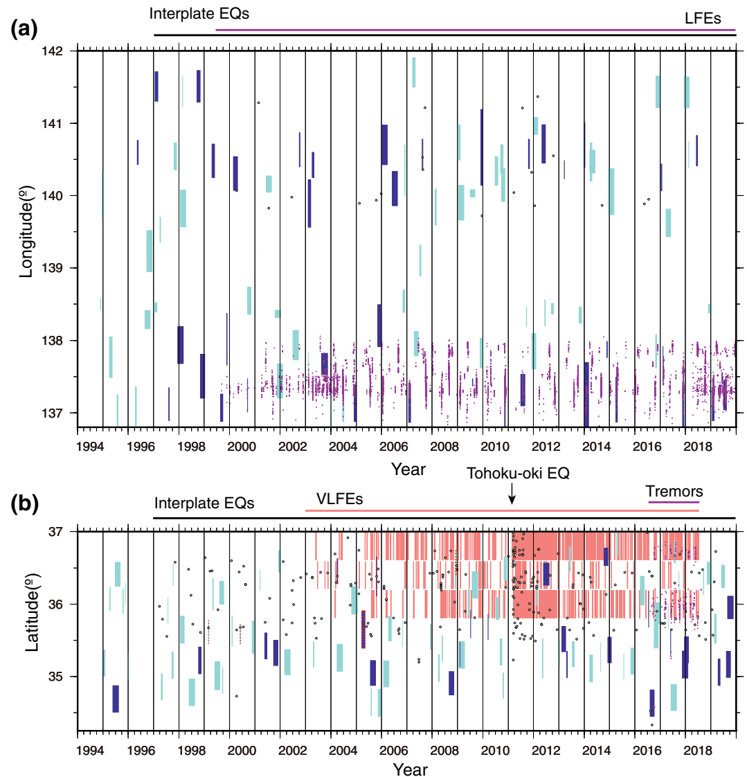
Figure 9. Space-time plot of detected SSEs. Blue and light-blue rectangles indicate the spatial extents and durations of probable and possible SSEs, respectively. Open circles indicate the centroids of the M_w \geq 4.8 interplate earthquakes whose focal mechanisms were determined by NIED. (a) SSEs along the Sagami and the Suruga Troughs. The vertical axis indicates the longitudinal extent. Purple dots indicate LFE epicenters determined by JMA. (b) SSEs along the Japan Trench. The vertical axis indicates the latitudinal extent. Thin red bars indicate VLFs (Baba et al., 2020). Rectangles with red horizontal stripes indicate SSEs related to M_w \geq 5.8 interplate earthquakes. Purple dots indicate tremor epicenters determined by Nishikawa et al. (2019). Note that each catalog covers a limited temporal extent: interplate earthquakes (January 1997–), VLFs (January 2003–July 2018), LFEs (July 1999–), and tectonic tremors (August 2016–August 2018), as shown by horizontal bars over each subfigure. NIED, National Research Institute for Earth Science and Disaster Prevention; SSE, slow slip event; VLFE, very low frequency earthquake.
