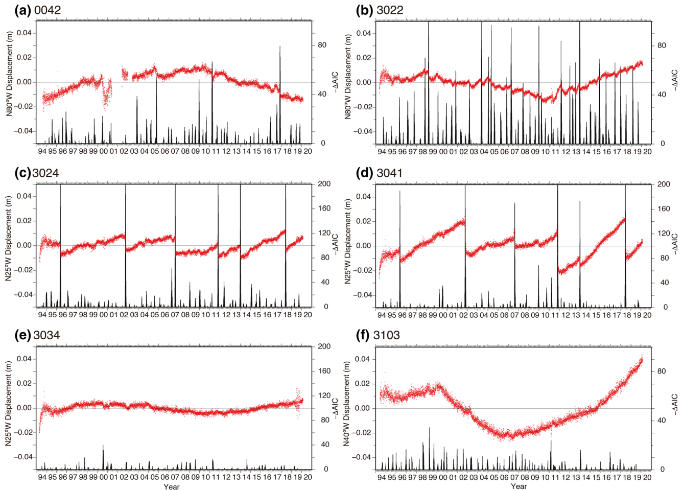
Figure 2. Cleaned coordinates at the selected GNSS stations. See Figure 1 for station locations labeled a-f. A linear trend was removed for plotting. (a) Daily coordinates (red dots) and -\Delta\text{AIC} (vertical black bars) for the \text{N}80^\circ\text{W} component at station 0042. (b) Same as (a), but for station 3022. (c) Same as (a), but for the \text{N}25^\circ\text{W} component at station 3024. (d) Same as (c), but for station 3041. (e) Same as (c), but for station 3034. (f) Same as (a), but for the \text{N}40^\circ\text{W} component at station 3103. AIC, Akaike Information Criterion; GNSS, Global Navigation Satellite System.
