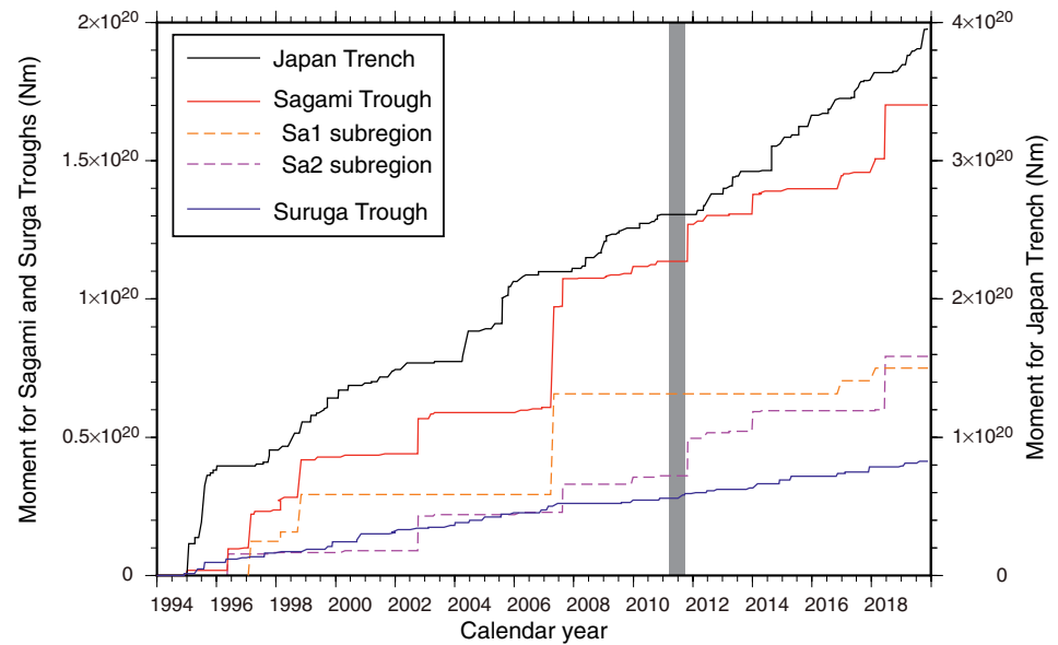
Figure 10. Moment release evolution of the detected SSEs. Note that the moment vertical scale is different for the Suruga and Sagami Troughs and the Japan Trench. Shading indicates the lower detection ability due to large postseismic displacements for 6 months following the Tohoku-oki earthquake. SSE, slow slip event.
