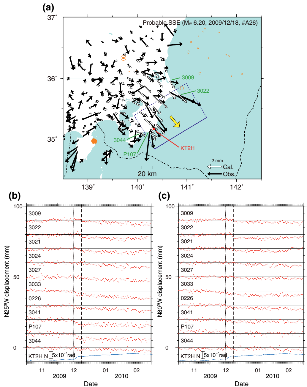
Figure 11. An SSE that occurred around December 18, 2009. It is likely that slow slip successively occurred along both the Sagami Trough and the Japan Trench (See text). (a) An estimated single rectangular fault model (dotted rectangle) along the Sagami Trough. The solid line of the rectangular fault and the yellow arrow indicate the shallow edge and the slip vector, respectively. The green characters indicate the GNSS stations whose time series are plotted in (b) and (c). KT2H is a borehole tiltmeter station. (b) GNSS time series in the N25°W direction, parallel to interplate slip along the Sagami Trough. The time series are arranged from the northeastern stations to the southwest stations along the coast. The bottom blue line shows the northward component of tilt at KT2H (NIED, 2010a). (c) GNSS time series in the N80°W direction, parallel to interplate slip along the Japan Trench. GNSS, Global Navigation Satellite System; NIED, National Research Institute for Earth Science and Disaster Prevention; SSE, slow slip event.
