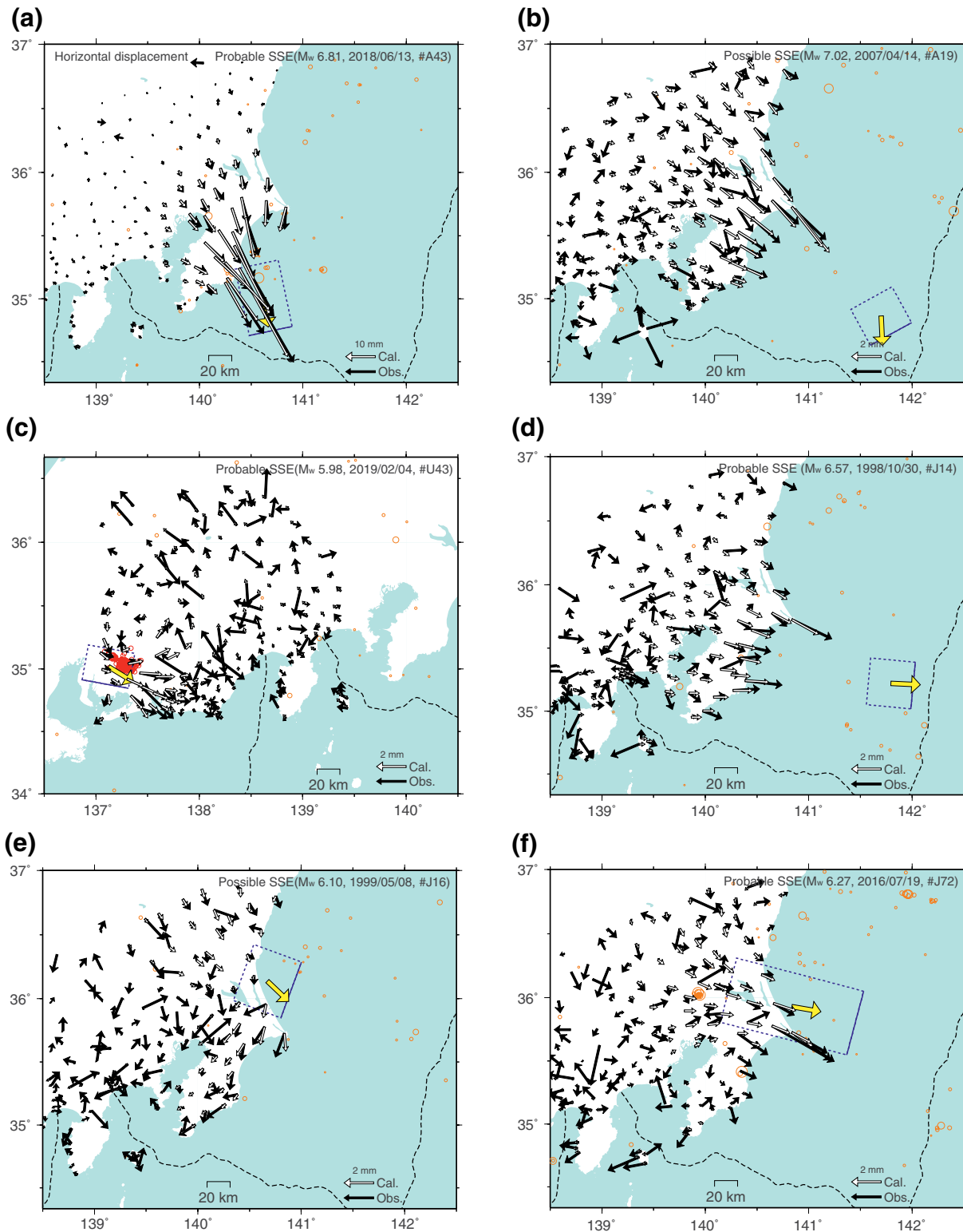
Figure 3. Examples of estimated SSE fault models. Blue dotted rectangles represent the estimated rectangular faults with yellow slip vectors. Solid lines of the rectangular faults represent the shallow edges. Black and white vectors represent observed and calculated displacements. Orange and red circles represent epicenters of regular ( M > 2 ) and LFEs that occurred within 5 days whose central dates are indicated. (a) Probable event on June 13, 2018. (b) Possible event on April 14, 2007. (c) Probable event on February 4, 2019. (d) Probable event on October 30, 1998. (e) Possible event on May 8, 1999. (f) Probable event on July 19, 2016. LFE, low frequency earthquake; SSE, slow slip event.
