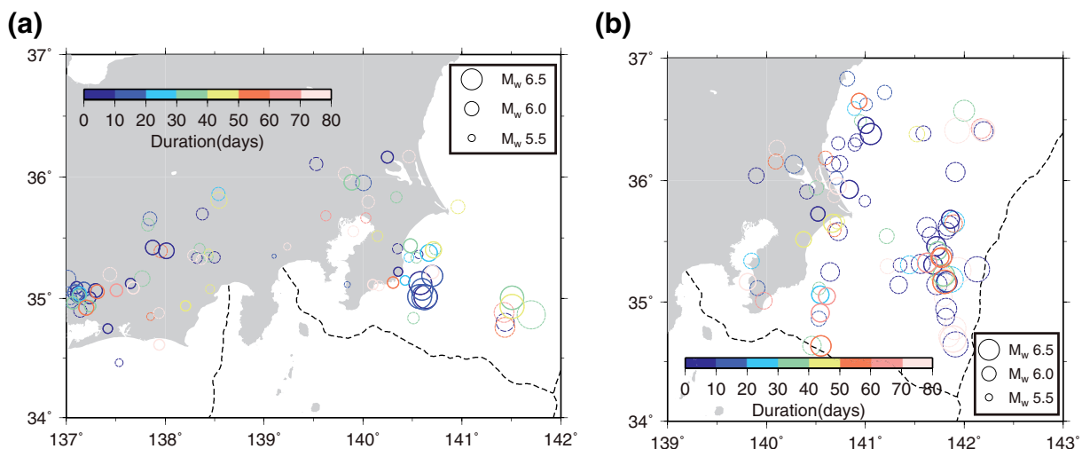
Figure 6. Duration for all detected SSEs. Circles with solid and broken lines indicate probable and possible SSEs, respectively. (a) Duration of detected SSEs along the Suruga and Sagami Troughs (b) Same as (a), but along the Japan Trench. SSE, slow slip event.
