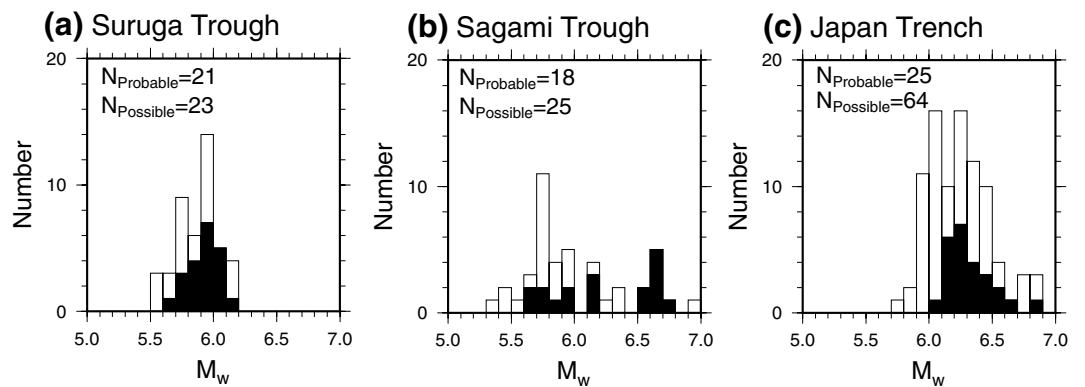
Figure 8. Moment magnitude histograms of estimated SSEs in three regions. Solid and open bars indicate the number of probable and possible SSEs, respectively. (a) Along the Suruga Trough. (b) Along the Sagami Trough. (c) Along the Japan Trench. SSE, slow slip event.
