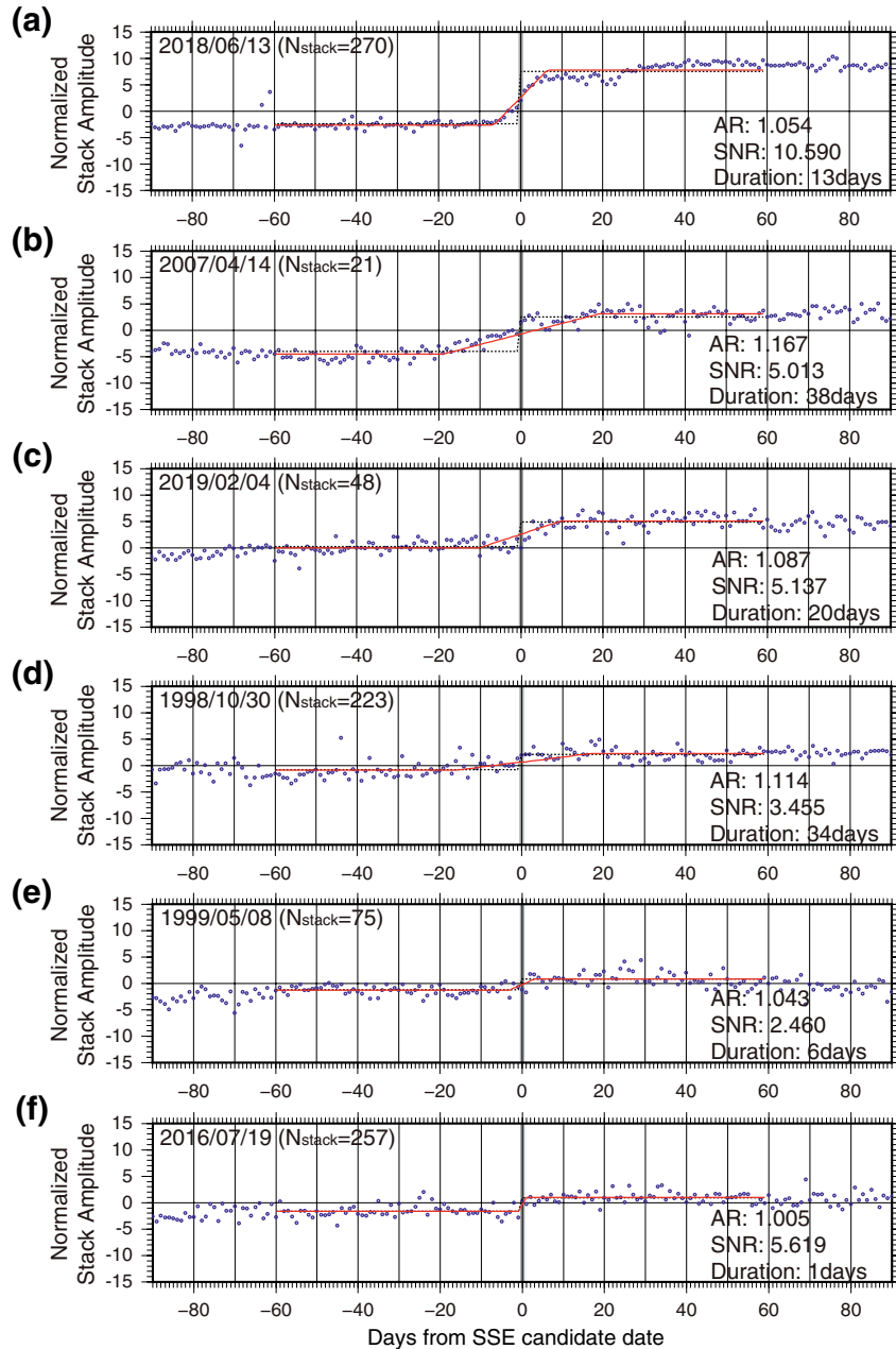
Figure 4. Examples of the stacked coordinate time series. Blue dots are the stacked GNSS time series. Red and black dotted lines are the best fit ramp and Heaviside functions, respectively. The central date of each time window is indicated as the referred SSE candidate date. N_{\text{stack}} , AR, SNR, and duration represent the number of stacked components, the amplitude ratio of the best fit ramp and Heaviside functions, the signal-to-noise ratio of the stacked time series, and the duration of the best fit ramp function, respectively. (a–f) correspond to the fault models in Figure 3, respectively. GNSS, Global Navigation Satellite System; SNR, signal-to-noise ratio; SSE, slow slip event.
