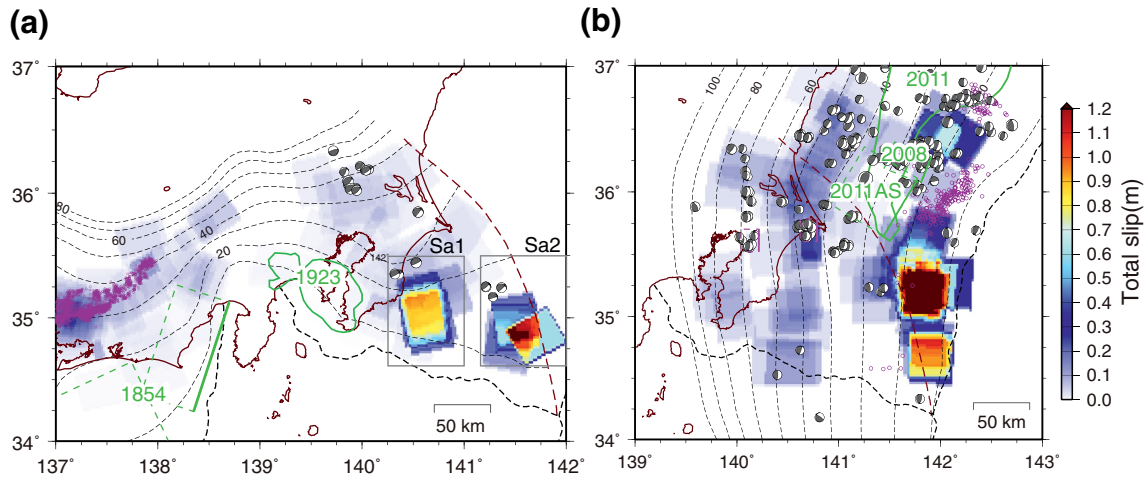
Figure 7. Cumulative slip distributions of SSEs from July 1994 to November 2019. Green areas and rectangles indicate the source areas of past megathrust earthquakes with their occurrence years. Purple dots and circles indicate epicenters of tectonic tremors (Nishikawa et al., 2019; Obara et al., 2010). Focal mechanisms of M_w \geq 4.8 interplate earthquakes from 1997 to 2019 determined by NIED are also plotted. (a) Slip along the Suruga and Sagami Troughs. Gray rectangles Sa1 and Sa2 indicate the regions used for plotting moment evolutions (Figure 10). (b) Slip along the Japan Trench. NIED, National Research Institute for Earth Science and Disaster Prevention; SSE, slow slip event.
