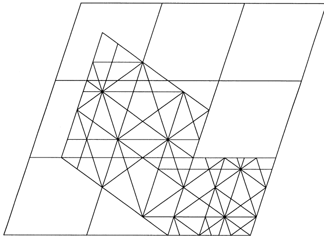
図 9: 5-fold sofic case
