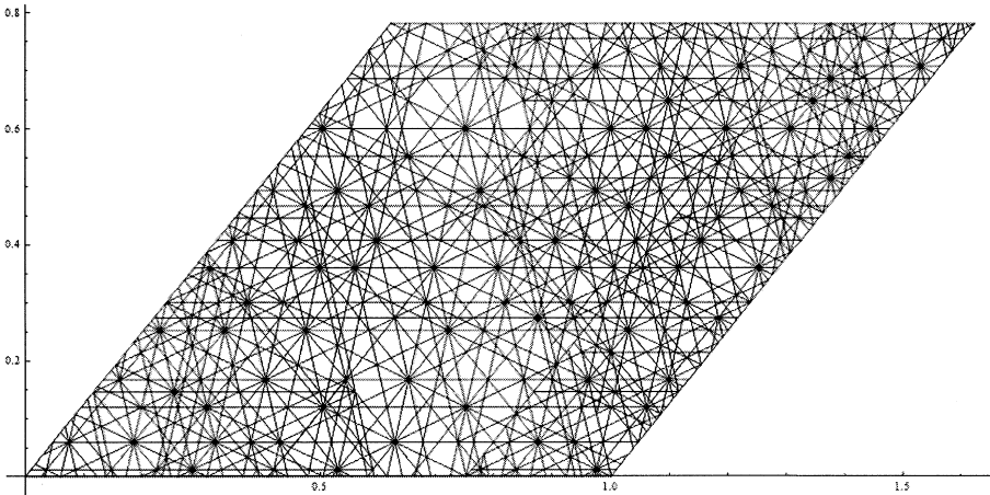
⊠ 10: Sofic 7-fold rotation
