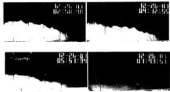
Fig. 1 Transformation processes of the head of a turbidity current (see Ashida et al., 1982)
