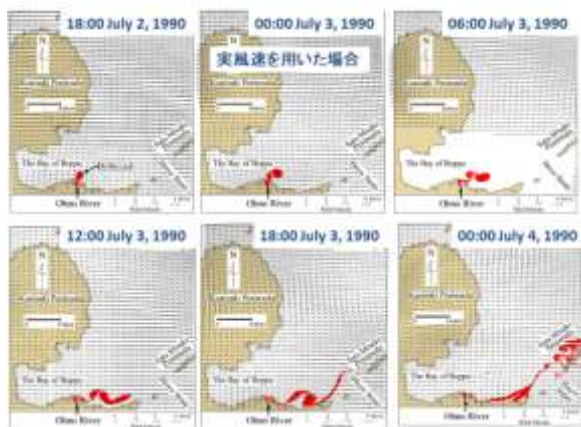
Fig. 4 Simulated positions of the driftwood (red dots) in case of using actual wind data
