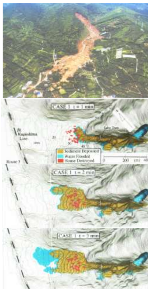
Fig. 5 Top photo is a deep-seated landslide and resultant debris flow deposited area at Harihara district. Bottom three figures are simulated sediment deposited and water inundated area.
