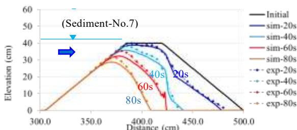
Fig. 7 Comparison between experimental and simulated erosion process of embankment due to overtopping of water
