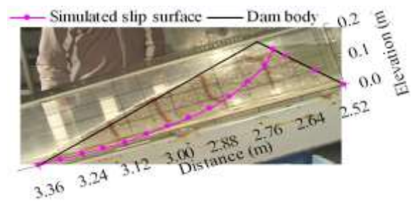
Fig. 8 Comparison between simulated and experimental slip surfaces generated in the natural dam body by gradually supplying water upstream
