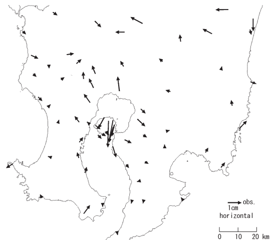
Fig. 5 Horizontal displacement of GNSS stations after reductions for influence of tectonic movement and activity of Kirishima volcano complex.
