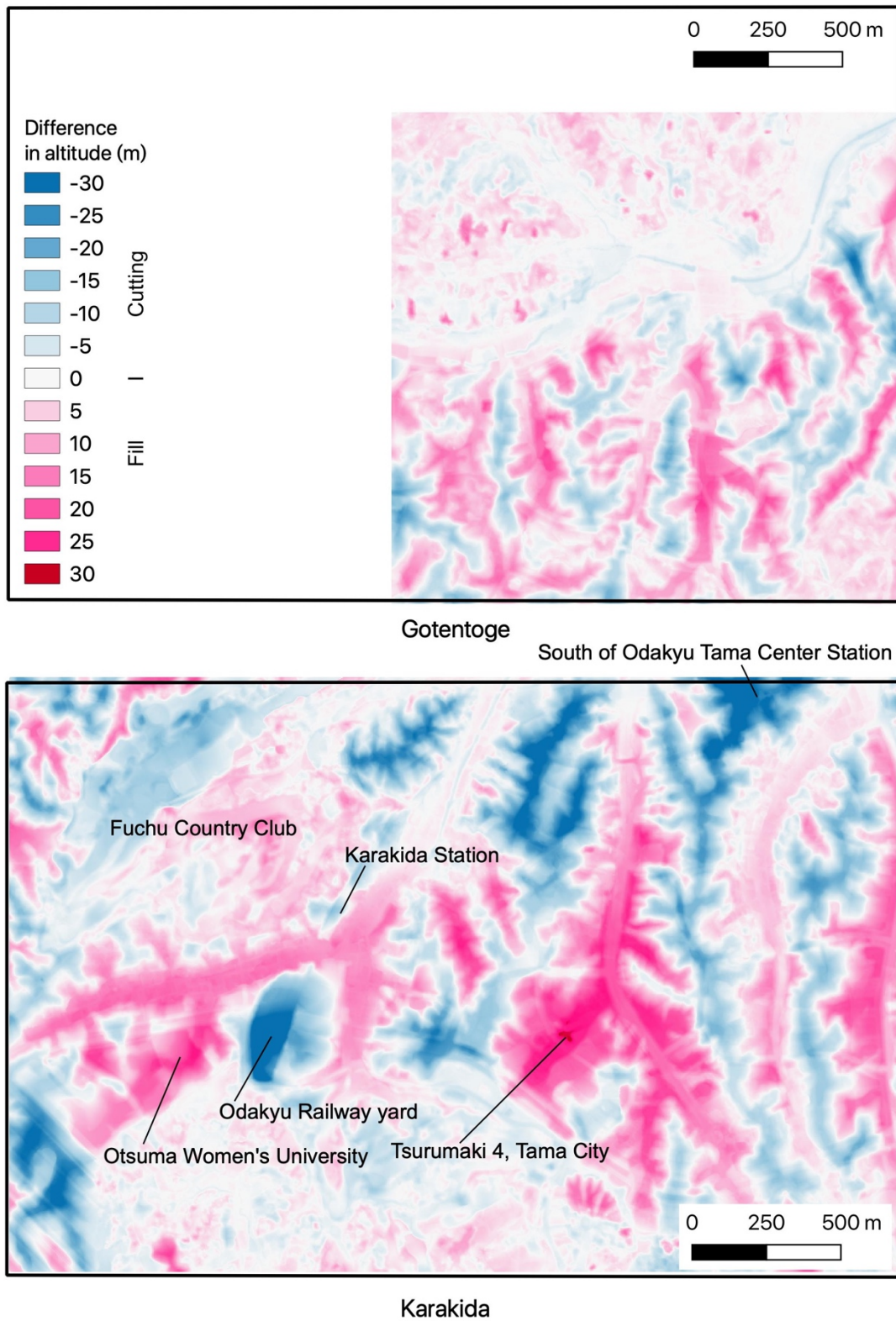
Fig. 9 Difference in altitude before and after the cutting and fill operation
