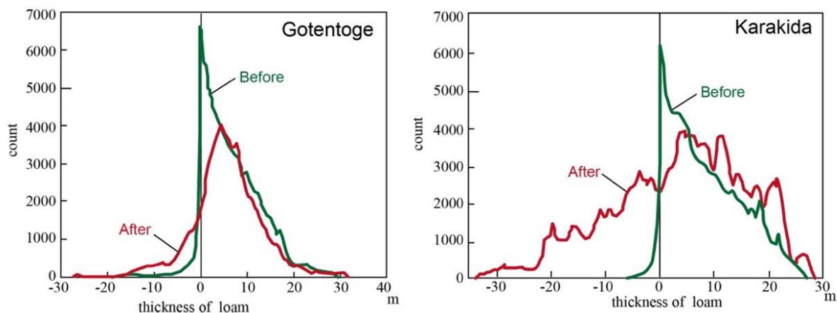
Fig. 13 Histogram of distribution of loam thickness before and after the cutting and fill operation
