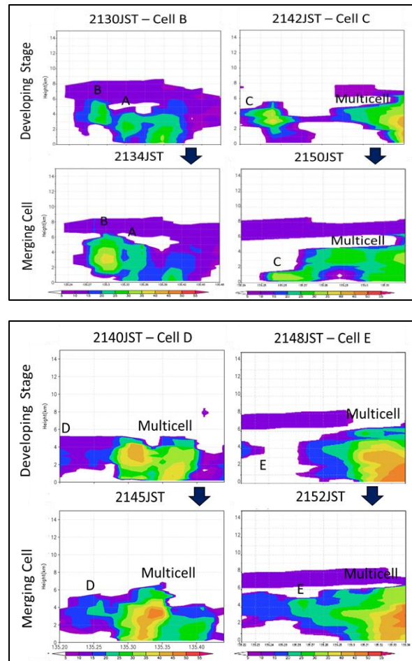
Fig. 7 The vertical cross-section of new cells for Z_h at the developing stage and merging cells
