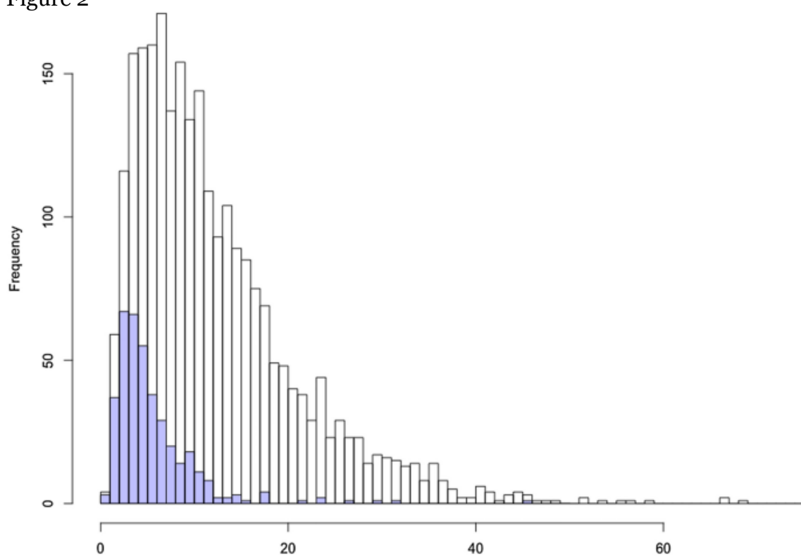
Distribution of inter-individual distances in a group of horses. White bars are data for all pair combinations in the group. Purple bars are data for nearest neighbors
