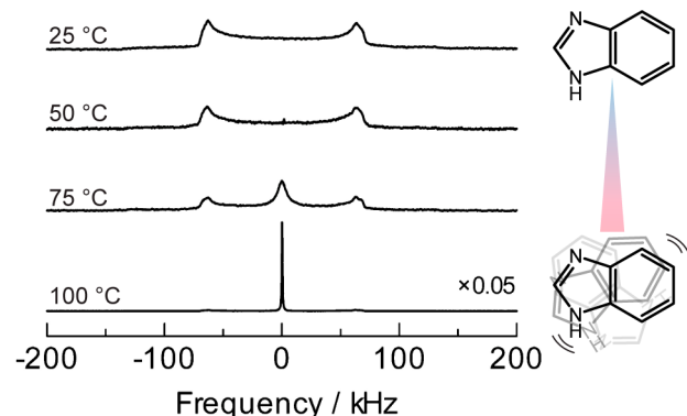
Figure 8. ^2\text{H} solid-state static NMR spectra of dehydrated [\text{Zn}_3(\text{H}_2\text{PO}_4)_6(\text{H}_2\text{O})_3](\text{HbIm})\text{-HbIm-d}_4 at 25, 50, 75, and 100 ^{\circ}\text{C} ( T_m = 164\text{ }^{\circ}\text{C} ). Adapted with permission from ref 53. Copyright 2013 American Chemical Society.
