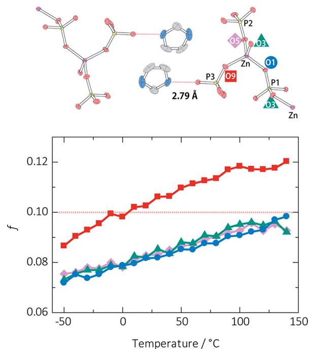
Figure 6. Degrees of thermal vibration of oxygen atoms around the \text{Zn}^{2+} . O1 (blue circles), O3 (green triangles), O5 (purple diamonds), and O9 (red squares). The ORTEP model of [\text{Zn}(\text{HPO}_4)(\text{H}_2\text{PO}_4)](\text{H}_2\text{Im})_2 at -50 °C and the H-bond distances are shown on the top. The Zn, P, O, N, and C atoms are shown in purple, yellow, red, blue, and gray, respectively; H atoms have been omitted. Adapted with permission from ref 26. Copyright 2015 American Chemical Society.
