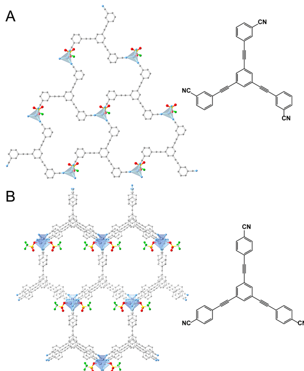
Figure 19. Crystal structures and ligands of (A) [Ag(mL1)(CF_3SO_3)] \cdot 2C_6H_6 and (B) [Ag(pL2)(CF_3SO_3)] \cdot 2C_6H_6 . Ag, C, N, O, F, and S atoms are represented by blue, gray, light blue, red, green, and yellow spheres, respectively.
