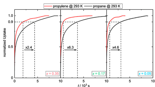
Figure 44. Kinetic sorption profiles of ZIF-62-blM x glass ( x = 0.05, 0.17, 0.35 ) recorded with an equilibrium pressure of \sim 54 kPa. Reprinted with permission from ref 116. Copyright 2019 American Chemical Society.
