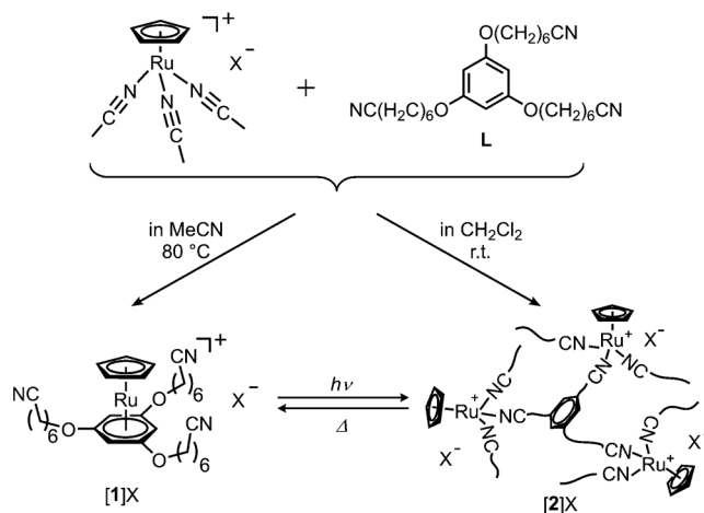
Figure 28. Reactions of [\text{Ru}(\text{C}_5\text{H}_5)(\text{MeCN})_3]\text{X} ( \text{X} = \text{FSA}^- , \text{PF}_6^- ) and L. Conversion between [1]\text{X} and [2]\text{X} occurs for \text{X} = \text{FSA}^- . Reprinted with permission from ref 173. Copyright 2016 The Royal Society of Chemistry.
