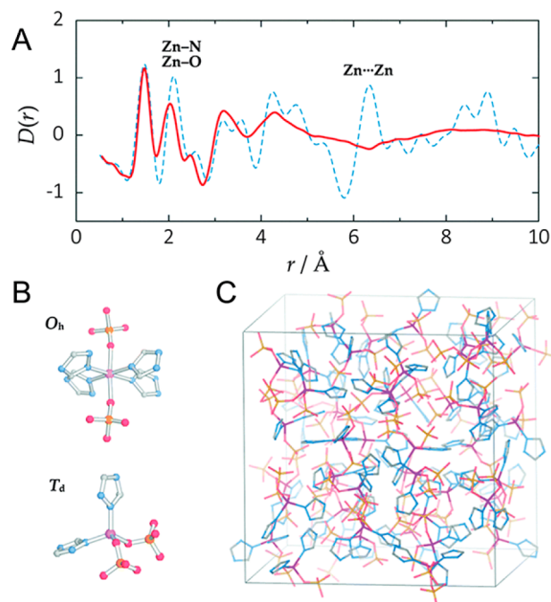
Figure 9. (A) Comparison of the D(r) of crystalline \text{Zn}(\text{HTr})_2(\text{H}_2\text{PO}_4)_2 (blue) and MQG (red) in the range 1–10 \text{\AA} (25 ^{\circ}\text{C} ). Some of the assigned peaks of the D(r) are indicated. (B) Arrangements around the \text{Zn}^{2+} for \text{Zn}(\text{HTr})_2(\text{H}_2\text{PO}_4)_2 (top) and its MQG (bottom, postulated). (C) The RMC amorphous cell comprises 50 \text{T}_d models for the MQG. \text{O}_h and \text{T}_d represent octahedral and tetrahedral geometry. Reprinted with permission from ref 54. Copyright 2015 The Royal Society of Chemistry.
