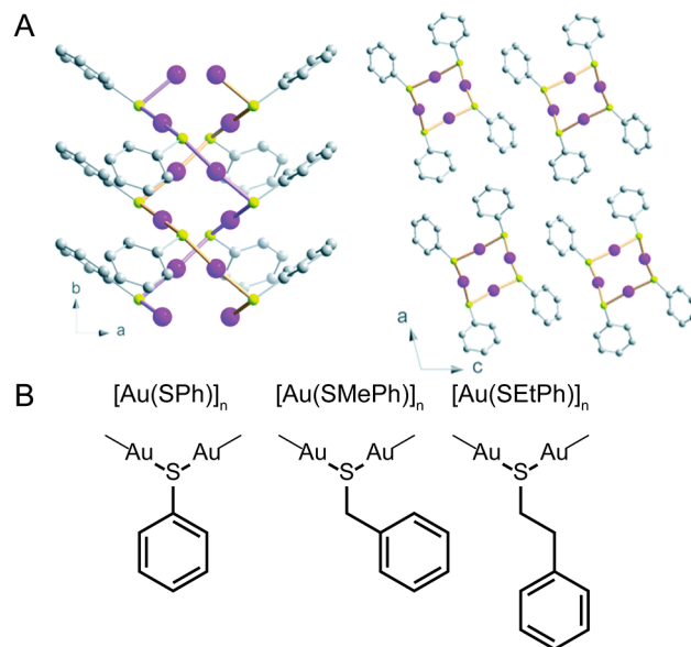
Figure 27. (A) Crystal structure of 1D \text{Au}(\text{SPh}) . Pink, yellow and gray spheres represent gold, sulfur and carbon atoms, respectively. (B) Representation of \text{Au}(\text{SPh}) and two other related CPs. Reprinted with permission from ref 34. Copyright 2020 The Royal Society of Chemistry. https://creativecommons.org/licenses/by/3.0/ .
