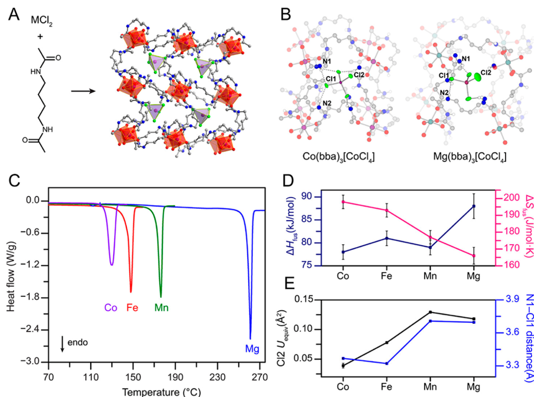
Figure 21. (A) Crystal structure of the 3D \text{Co(bba)}_3[\text{CoCl}_4] . Note that the bba ligand is disordered over two positions, and only the higher occupancy atomic positions are shown. Purple, red, gray, blue, and green spheres represent Co, O, C, N, and Cl atoms, respectively; H atoms have been omitted for clarity. (B) Comparison between the geometry of hydrogen bonds with [\text{CoCl}_4]^{2-} for \text{Co(bba)}_3[\text{CoCl}_4] and \text{Mg(bba)}_3[\text{CoCl}_4] at -173^\circ\text{C} to highlight the additional set of moderate hydrogen-bonding interactions present in the former compound. Teal spheres represent Mg atoms, and only N–H protons are shown. (C) DSC traces for \text{M(bba)}_3[\text{M}'\text{Cl}_4] compounds ( \text{M}/\text{M}' = \text{Co}, \text{Fe}, \text{Mn} ; and \text{M} = \text{Mg}, \text{M}' = \text{Co} ) with a heating rate of 5^\circ\text{C min}^{-1} for all compounds. (D) Trends of difference in enthalpy ( \Delta H_{\text{fus}} ) and entropy ( \Delta S_{\text{fus}} ) of fusion between solid and liquid phases for \text{Co(bba)}_3[\text{CoCl}_4] , \text{Fe(bba)}_3[\text{FeCl}_4] , \text{Mn(bba)}_3[\text{MnCl}_4] , and \text{Mg(bba)}_3[\text{CoCl}_4] . (E) Equivalent isotropic displacement parameters, U_{\text{equiv}} of Cl2 atoms and N1–Cl1 hydrogen bond donor–acceptor distances at -173^\circ\text{C} , generally correlated with each other and inversely correlated with \Delta S_{\text{fus}} . Reprinted with permission from ref 41. Copyright 2021 American Chemical Society.
