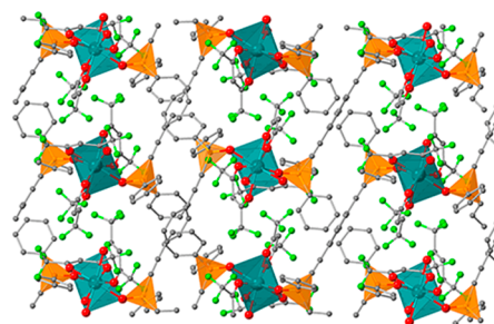
Figure 36. Crystal structure of Eu(hfa) 3 (p-dpeb). Eu, C, P, O, and F atoms are represented by teal, gray, orange, red, and green spheres, respectively.
