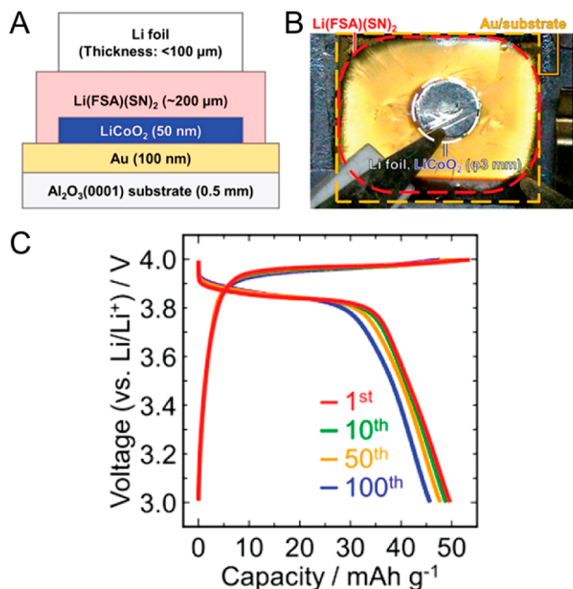
Figure 35. (A) Cell configuration and (B) top-view photograph of Li-battery (LiLi[N(SO 2 F) 2 ] 2 (NCCH 2 CH 2 CN) 2 |LiCoO 2 |Au). (C) Charge–discharge profiles at a current density of 1 μA cm -2 . Reprinted with permission from ref 30. Copyright 2021 American Chemical Society.
