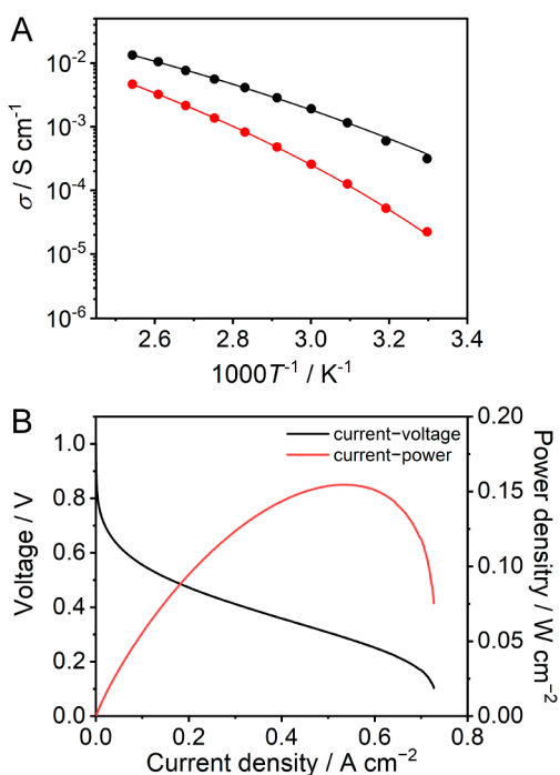
Figure 33. (A) H + conductivity as a function of temperature under anhydrous conditions of (dema) 0.35 [Zn(H 2 PO 4 ) 2.35 (H 3 PO 4 ) 0.65 ] glass (black) and protic ionic liquid [dema][H 2 PO 4 ] (red). (B) I – V (black) and I – W (red) curves of a H 2 /O 2 fuel cell employing (dema) 0.35 [Zn(H 2 PO 4 ) 2.35 (H 3 PO 4 ) 0.65 ] glass as an electrolyte at 120 °C without humidification. Reprinted with permission from ref 31. Copyright 2020 The Royal Society of Chemistry. https://creativecommons.org/licenses/by/3.0/ .
