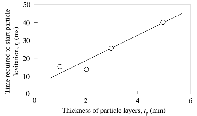
Fig. 9. Effect of thickness of particle layers on the time required to start particle levitation ( V_{down} = -4 kV, V_{up} = 4 kV)
