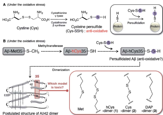
Fig. 1 (A) Mechanism of protein persulfidation through the formation of cysteine persulfide under the condition of oxidative stress. (B) A \beta 42 persulfidation hypothesis. Possible formation of persulfidated A \beta in the pathogenesis of AD using methyltransferase as a substrate of Met35-A \beta . Structure of hCys-dimer (1), Cys-dimer (2), and DAP-dimer (3) of E22P-A \beta 42 based on toxic dimer model of A \beta 42. 27
