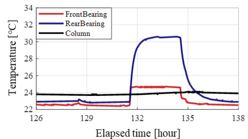
Fig. 5. Temperature history during warm-up.
