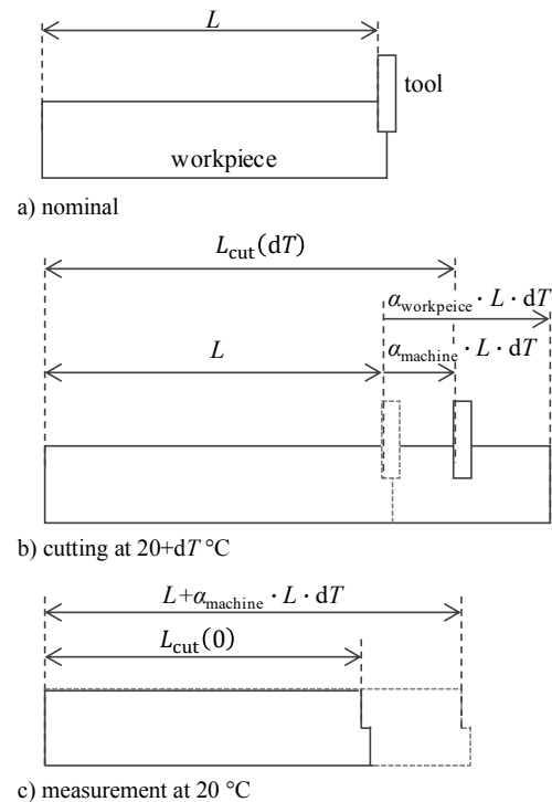
Fig. 2. Schematics of workpiece deformation around cutting at 20+dT °C.
