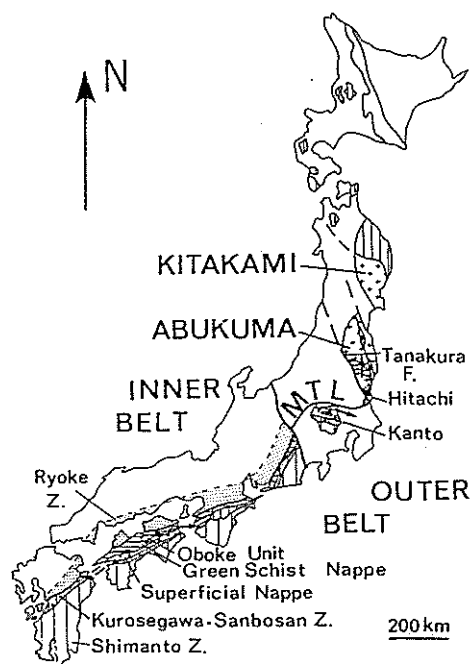
Fig. 6. General map of the Japanese Islands showing the Abukuma massif and the Ryoke zone. Arrows represent the average trend of the lineation in the Green Schist nappe of Southwest Japan and in the Hitachi and Gosaisho Groups (Faure, et al., 1986).
