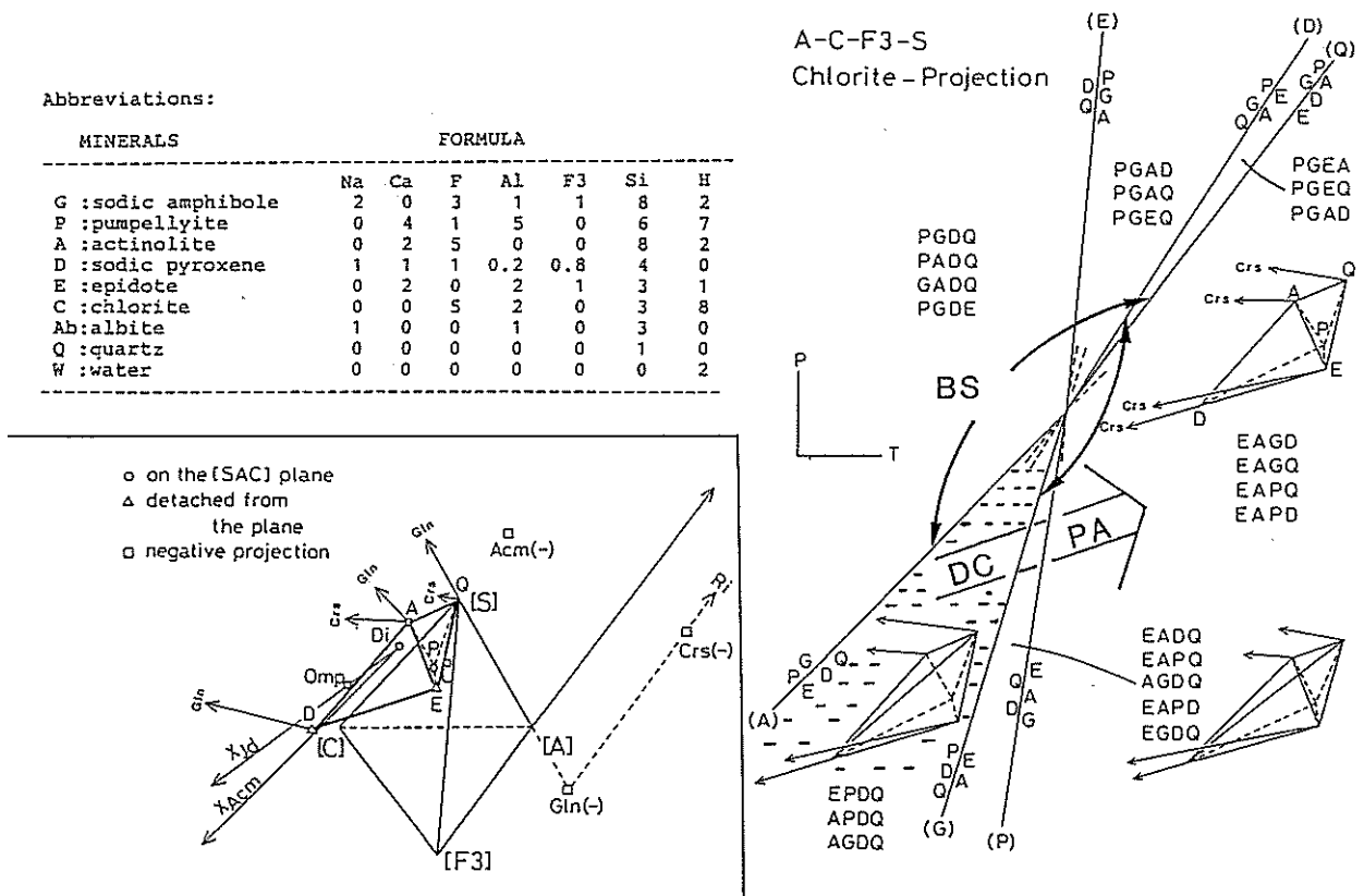
Fig. 35. Petrogenetic grid for the ACF3-S system with six phases. BS: Blue (glaucophan) schist facies, PA: Pumpellyite-actinolite facies, DC: Sodic pyroxene-chlorite facies.
