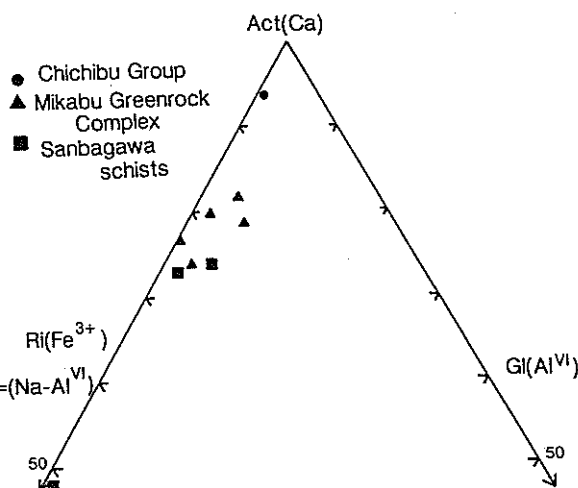
Fig. 30. Averaged compositions of actinolite in each geologic unit. Fe 3+ /Fe 2+ ratios of amphiboles are re-calculated on the basis of total cations = 13.0 in B, C, and T sites of amphibole formula (Leak, 1978).
