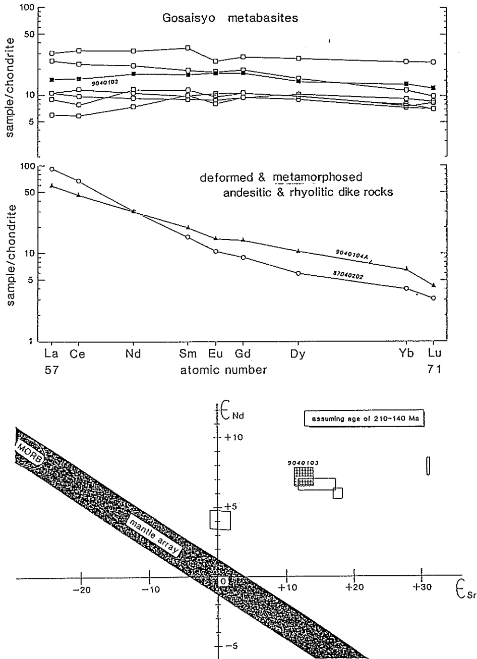
Fig. 12. Diagrams showing rare earth element and isotope (Nd, Sr) variations of Gosaisyo metabasite as well as deformed and metamorphosed andesitic and rhyolitic dike rocks (Hiroi et al., in prep.).
