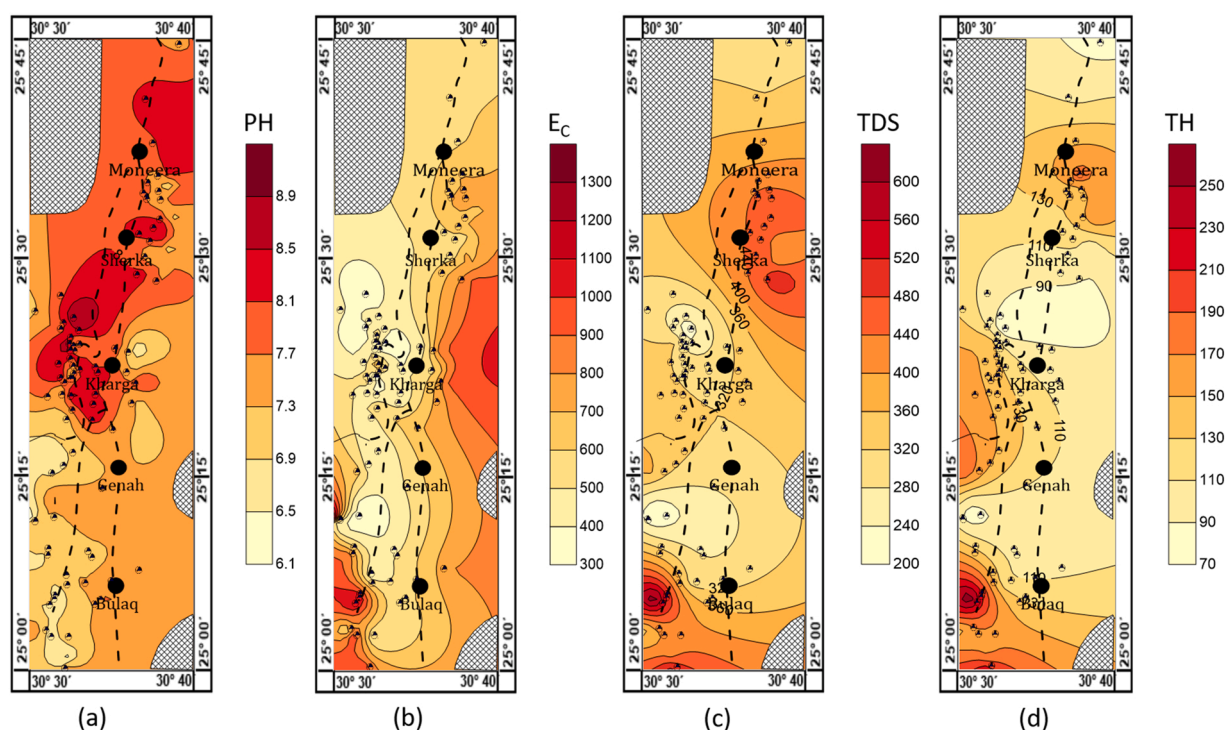
Fig. 2. Spatial distribution maps of a) pH, b) EC ( \mu\text{s}/\text{cm} ), c) TDS ( \text{mg}/\text{l} ), and d) TH ( \text{mg}/\text{l} as \text{CaCO}_3 ) in groundwater wells across the study area (the dashed lines represent roads).
