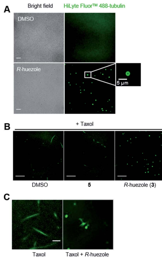
Fig. 4 Microscopic observation of the effects of R -huezole ( 3 ) on tubulin in vitro . (A) In vitro tubulin sequestration with R -huezole ( 3 ). Labeled tubulin (200 nM) was incubated with DMSO (1%) or R -huezole (50 \mu M) for 30 min before imaging. Scale bars, 10 \mu m. (B) Effects of R -huezole ( 3 ) on Taxol-induced tubulin polymerization in vitro . Labeled tubulin was dissolved in G-PEM buffer including Taxol (1 \mu M) followed by incubation with 50 \mu M R -huezole ( 3 ) for 30 min at 37 ^{\circ} C prior to imaging. Scale bars, 20 \mu m. (C) R -huezole-tubulin condensates under a highly polymerization-inducing condition. Polymerization of labeled tubulin (900 nM) was induced overnight by Taxol (50 \mu M) in the presence or absence of 50 \mu M R -huezole ( 3 ) in PBS. Scale bar, 5 \mu m.
