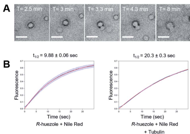
Fig. 3 Liquid-like phase separation of R -huezole ( 3 ). (A) Bright field time-lapse images of coalescing puncta of R -huezole ( 3 ). Scale bars, 5 \mu m. (B) FRAP assays of Nile-Red-doped R -huezole particles (90 nM Nile Red and 50 \mu M R -huezole). Recovery of the normalized fluorescence intensities indicated t_{1/2} values in the absence (9.88 s) and presence (20.3 s) of tubulin (200 nM). The blue lines indicate SEM, and the red lines show the results of exponential fitting with the average intensities of fluorescent particles ( N = 30 for Nile Red + R -huezole and N = 94 for Nile Red + R -huezole + tubulin, respectively).
