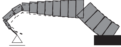
Figure 8: Deformed shape of optimal solution of Type 1 for Problem P4 with stress constraints with variable nodal locations; dotted line: undeformed shape.
