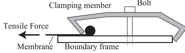
Figure 11: Illustration a clamping member with tension adjustment bolt.
