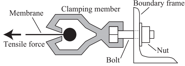
Figure 9: Illustration of the section of a self-fastening clamping member.
