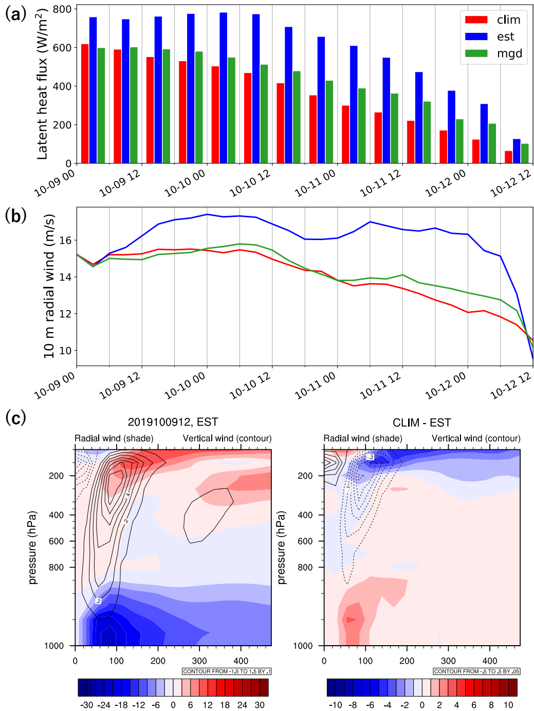
Fig. 7: (a) Latent heat flux ( W/m^2 ) and (b) 10 m radial wind (m/s) averaged within 200 km radius from TC center. (c) Azimuthal averaged radial wind (color, positive in outward) and vertical wind (contour, positive in upward) at 1200 UTC 9 October. Left panel shows EST experiment and right panel shows the difference of CLIM and EST.
