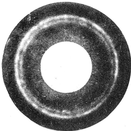
Photo. 7. Specimen H6, \sigma_a = \pm 16 , \sigma_m = -16 , N = 4 .
