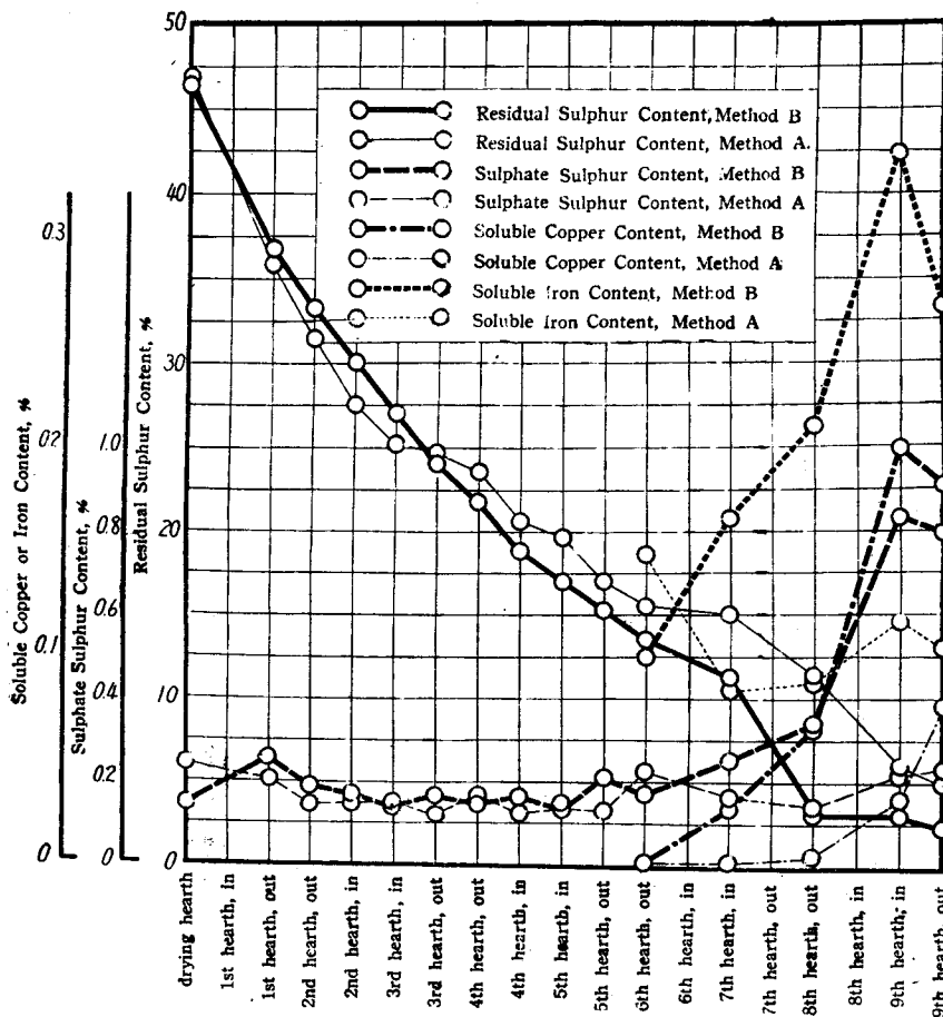
Fig. 8. Roasting Test of Nine Hearths Herreshoff Furnace. (Charging Rate 22 t/d)
