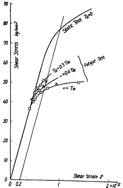
Fig. 21. Relation between the shear stress and strain in static and fatigue tests (SUP4).
