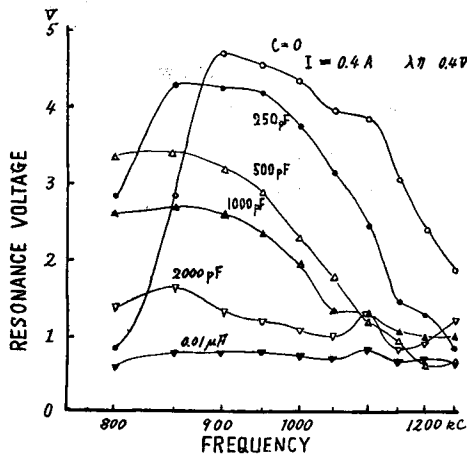
Fig. 5 Frequency response of DC discharge with interterminal capacitor.
