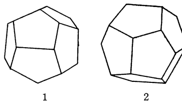
Fig. 7 Pentagonal dodecahedron
