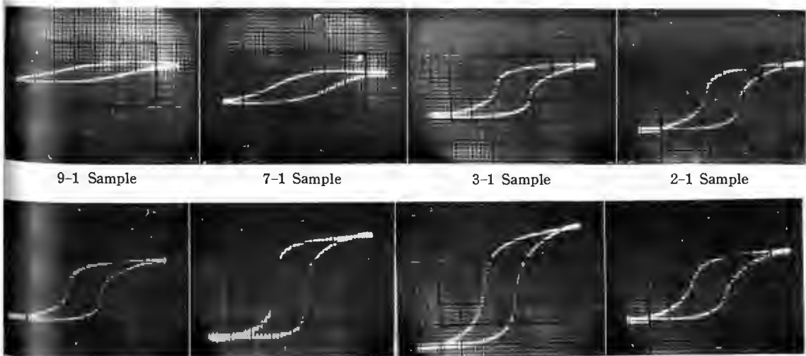
Fig. 3 Intensity of magnetization at various temperature
